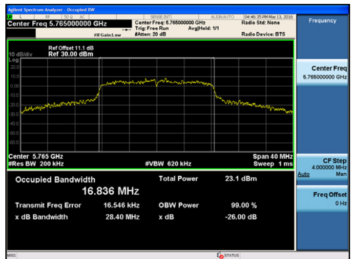
802.11a UNII 3 BAND 26dB Bandwidth (CH 153)
