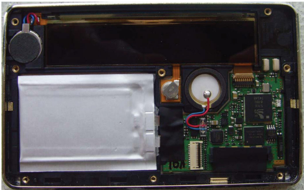
Bottom View of Transmitter
