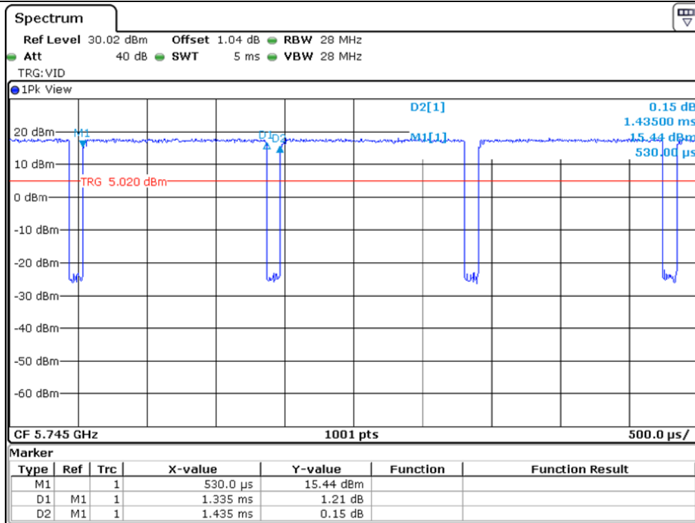
UNII 3_802.11 a
