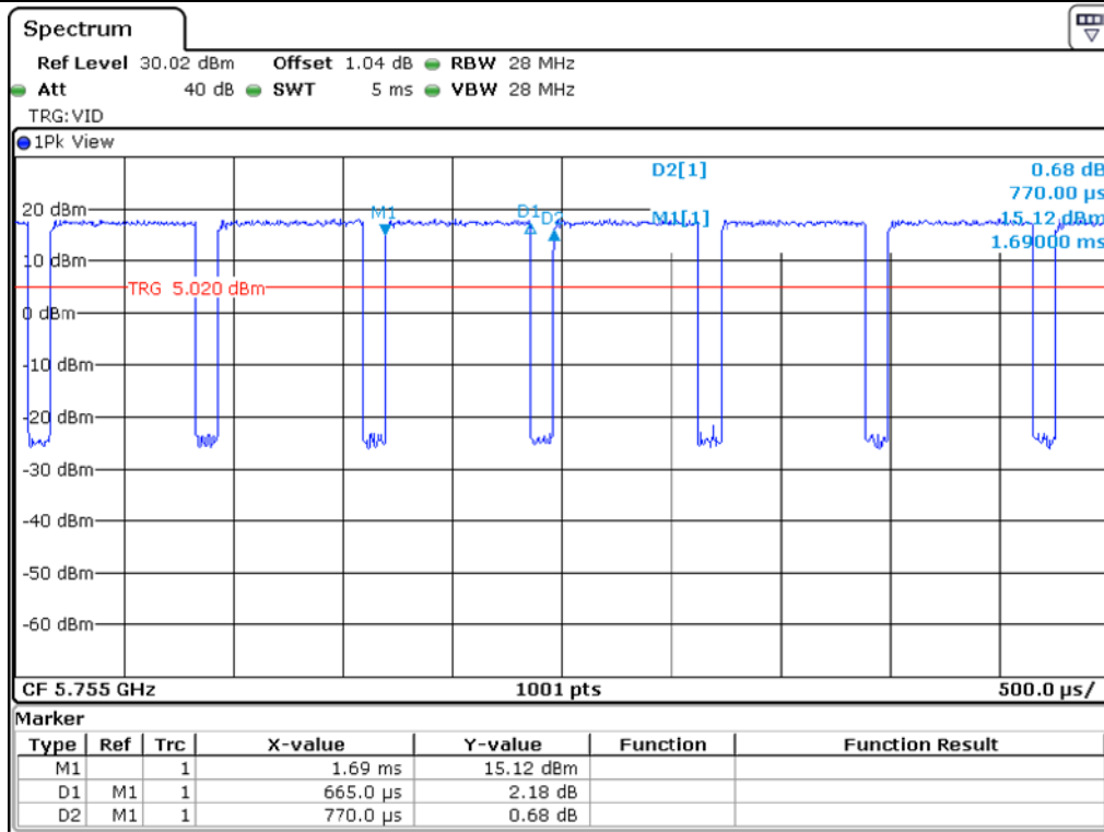
UNII 3_802.11 HT40
