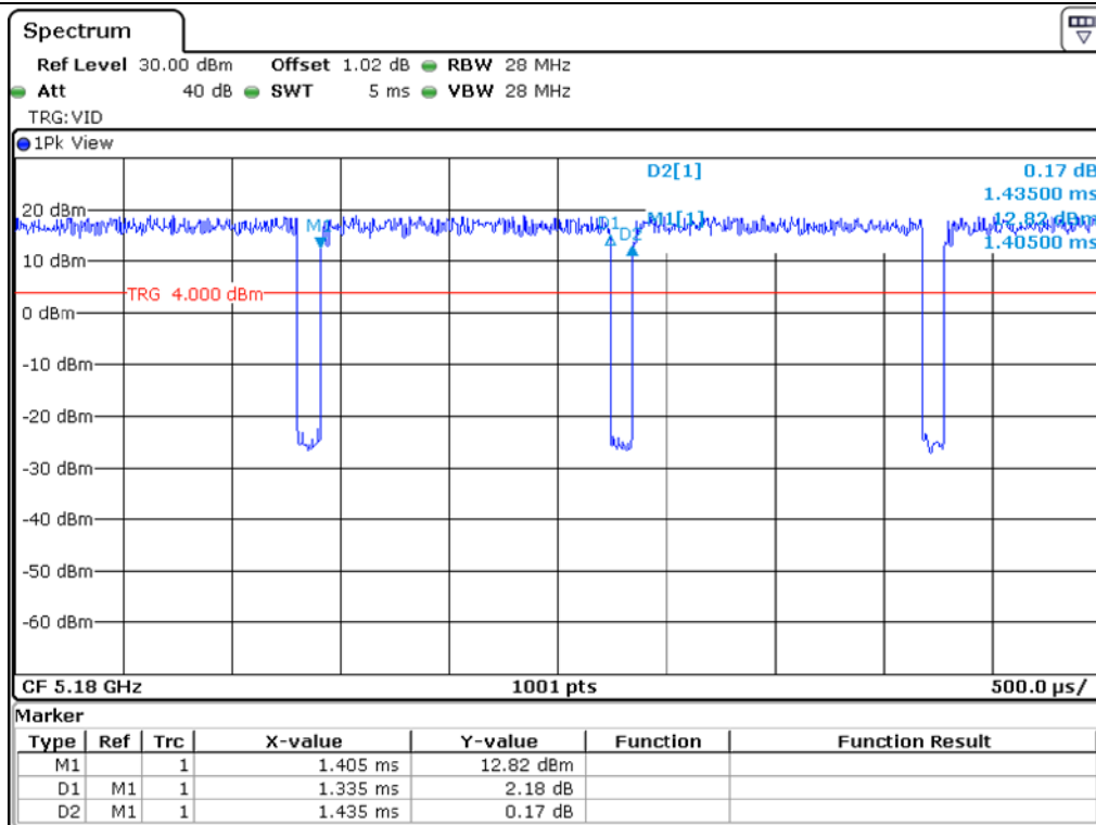
UNII 1_802.11 HT 20
