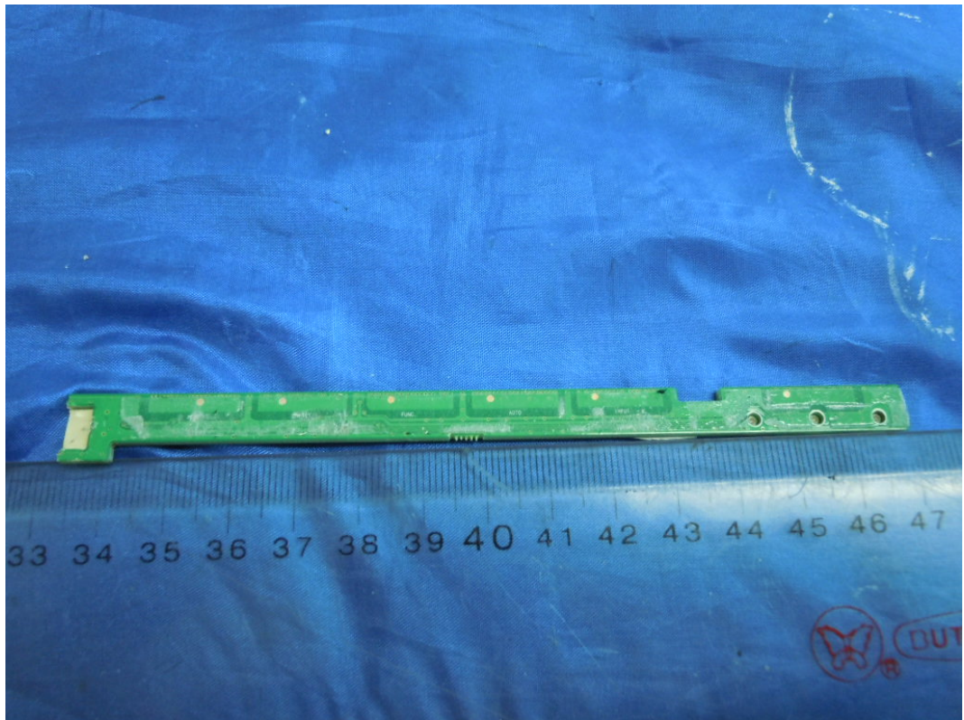
FIGURE 6 LCD MONITOR (M/N: IPS277LY) KEY BOARD (COMPONENT SIDE)
