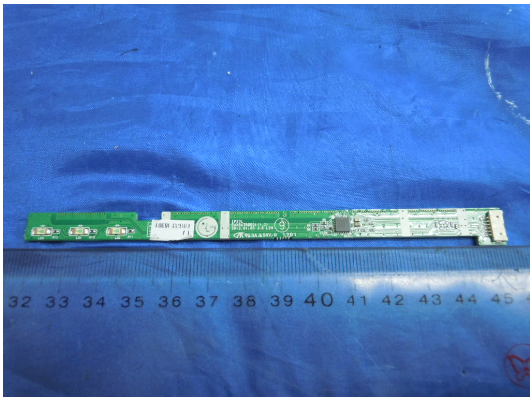
FIGURE 7 LCD MONITOR (M/N: IPS277LY) KEY BOARD (SOLDERED SIDE)
