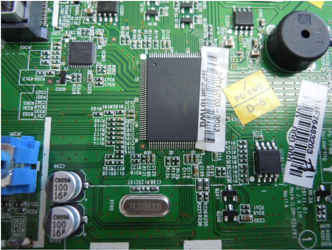
FIGURE 5 LCD MONITOR (M/N: IPS277LY) CRYSTAL ON MAIN BOARD
