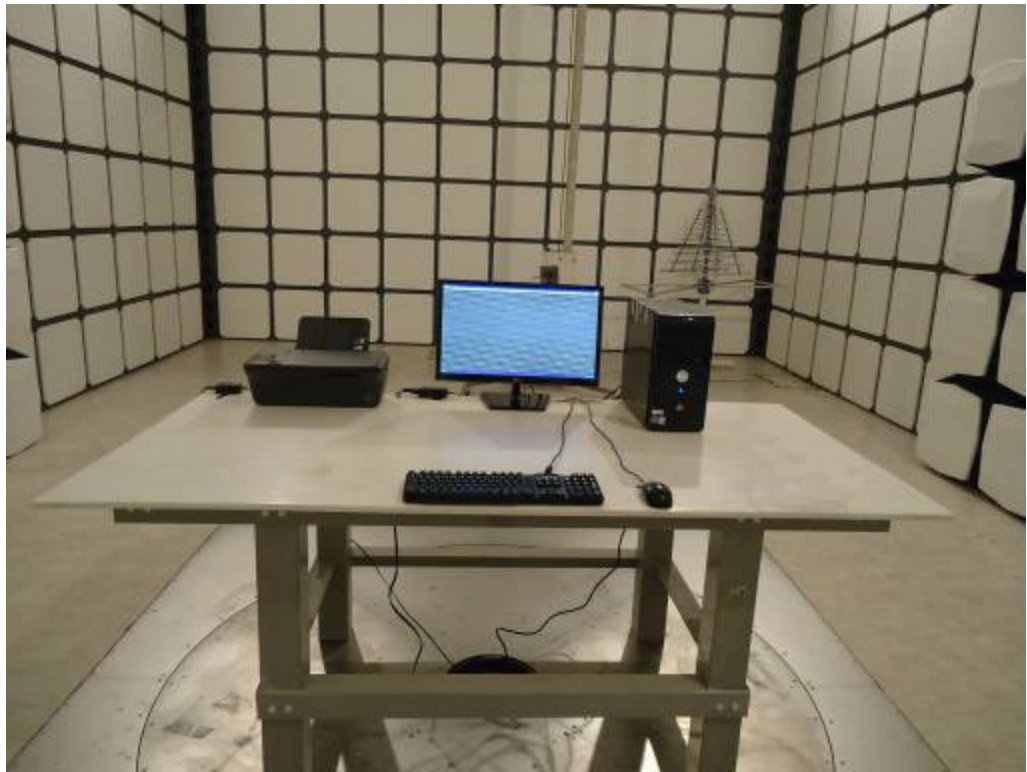
Front View of Radiated Emission Test (1000MHz ~ 18000MHz)
