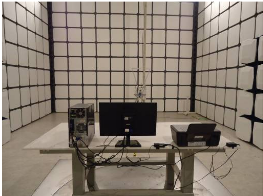
Back View of Radiated Emission Test (30MHz ~ 1000MHz)
