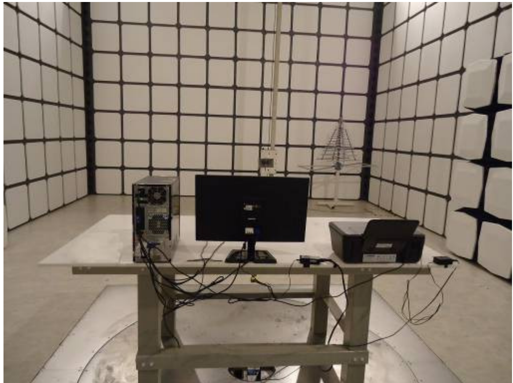
Back View of Radiated Emission Test (1000MHz ~ 18000MHz)
