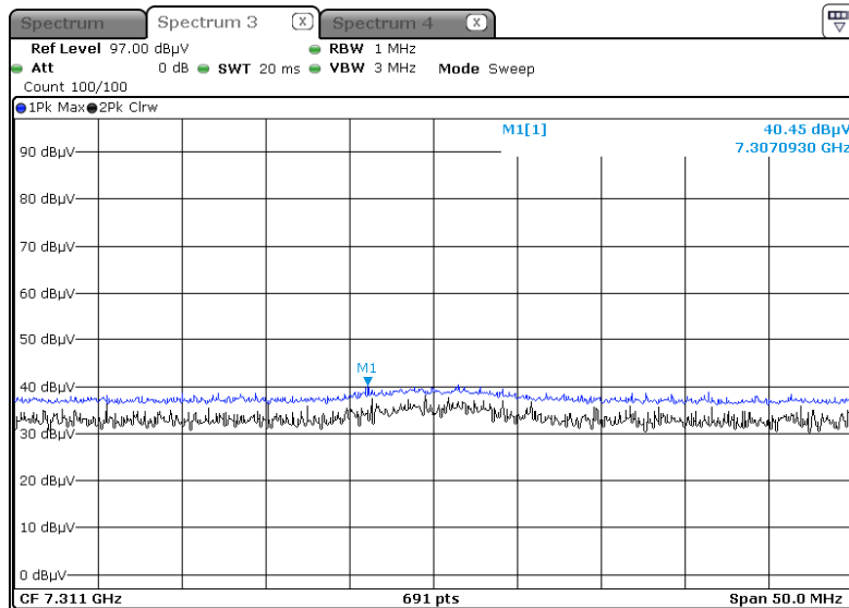
Radiated Spurious Emissions plot – Peak Measured Value (802.11b, Ch.6 3rd Harmonic)
