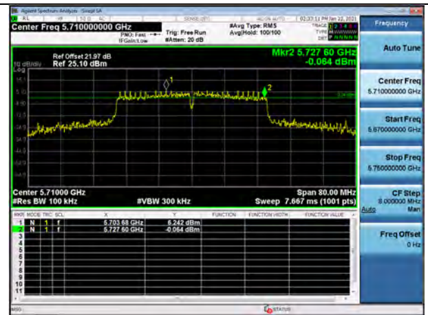
802.11ac_VHT40 CH.142
