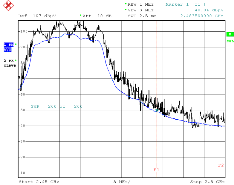
Radiated Restricted Band Edges plot – Average Reading (802.11g_Ch.11, Z-V)
