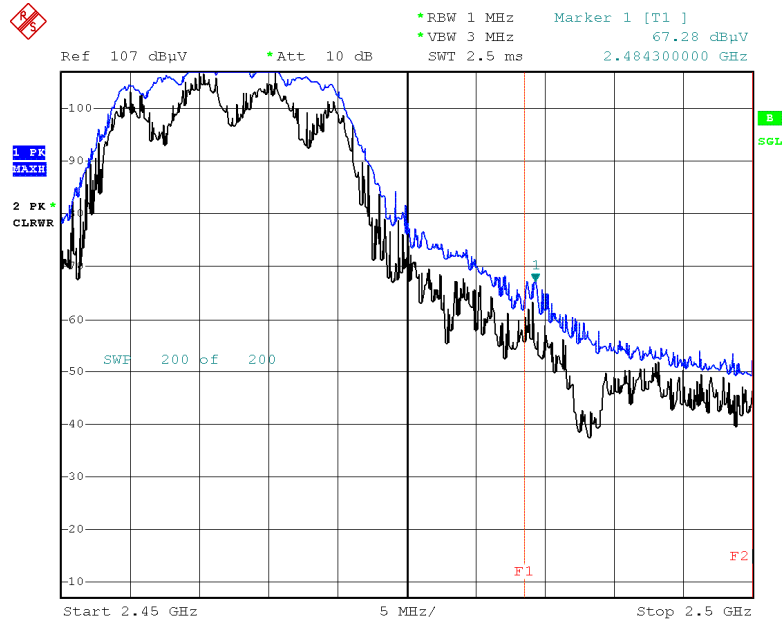
Radiated Restricted Band Edges plot – Peak Reading (802.11g_Ch.11, Z-V)
