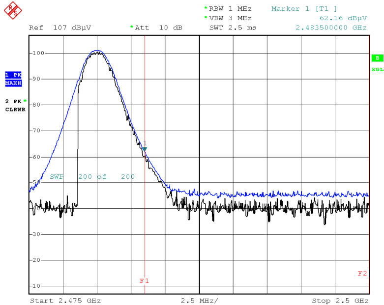
Radiated Restricted Band Edges plot – Peak Reading ( \pi/4 DQPSK, Ch.78, Z-V)
