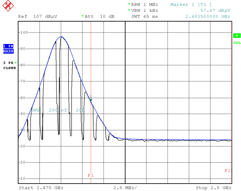
Radiated Restricted Band Edges plot – Average Reading ( \pi/4 DQPSK, Ch.78, Z-V)
