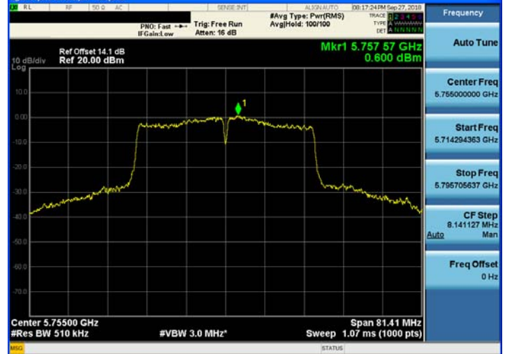
802.11ac_VHT40 UNII 3 BAND PSD CH 151
