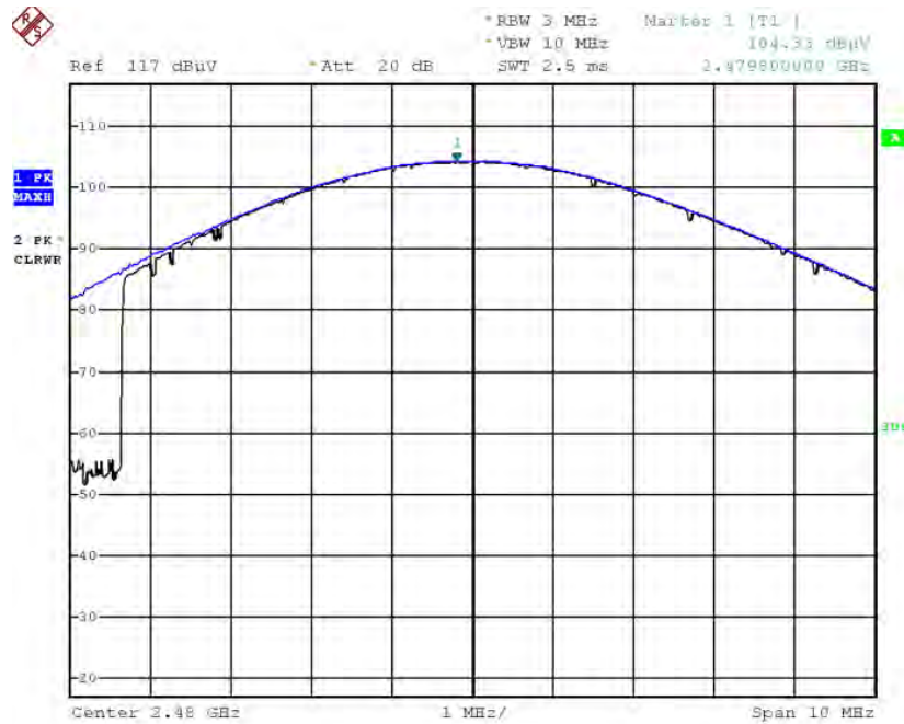
Radiated Power plot (GFSK, Ch78)
