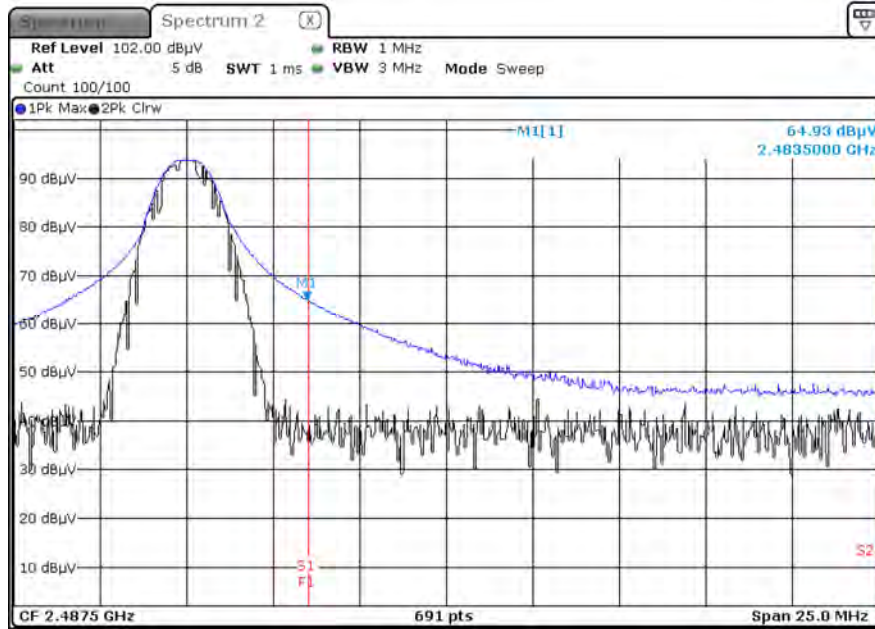
Radiated Restricted Band Edges plot – Average & Peak Result (GFSK, Ch.78, Y-V)
