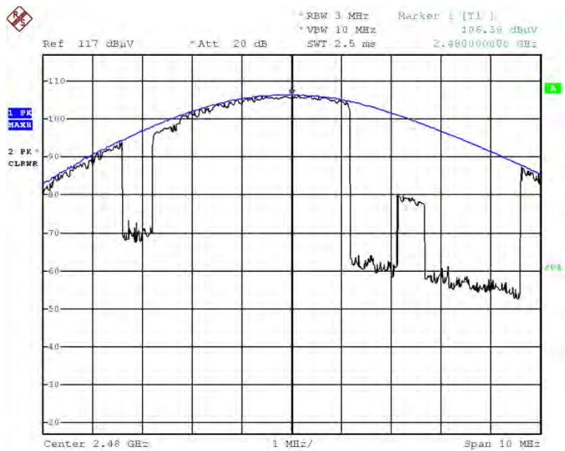
Radiated Power plot ( \pi/4 DQPSK, Ch78)
