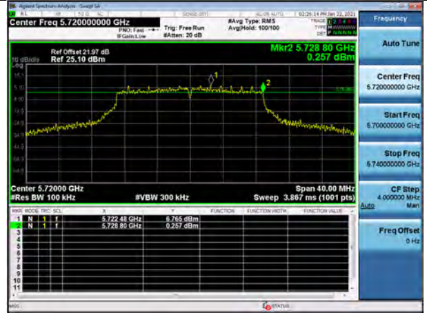
802.11ac_VHT20 CH.144
