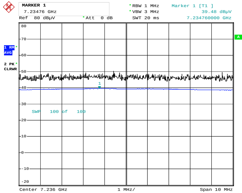
Radiated Spurious Emissions plot – Average Reading (802.11g, Ch.1 3rd Harmonic)
