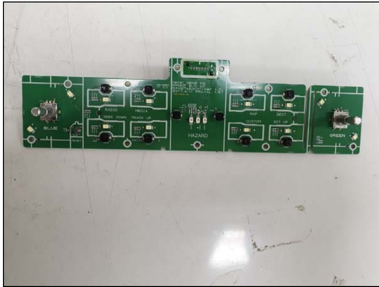
Top view of Sub PCB2
