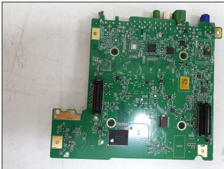
Bottom view of Sub PCB1
