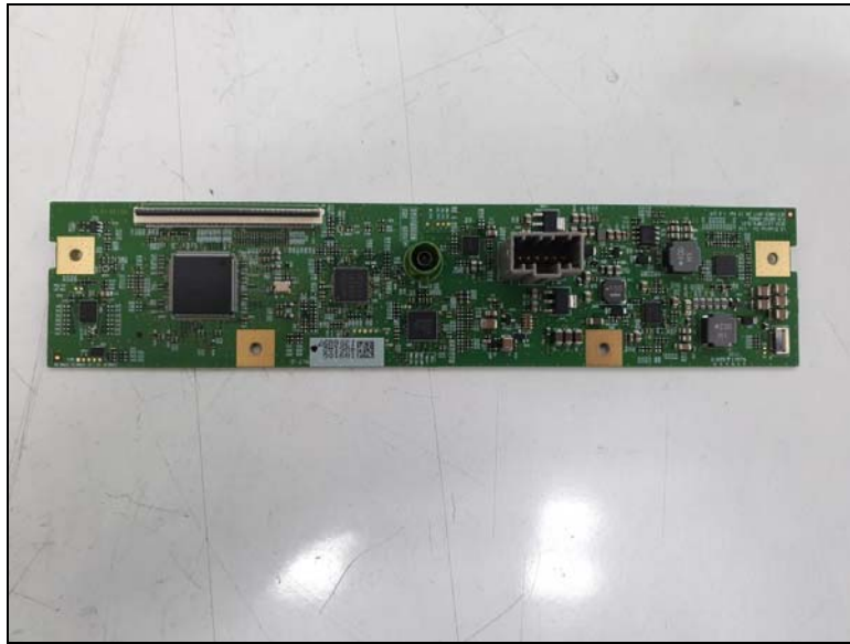
Top view of LCD PCB
