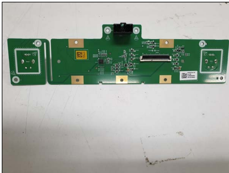
Bottom view of Sub PCB2
