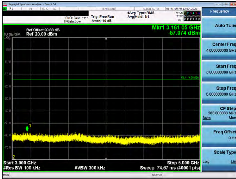
Conducted Spurious Emission (802.11g_Ch.6_6 Mbps)
