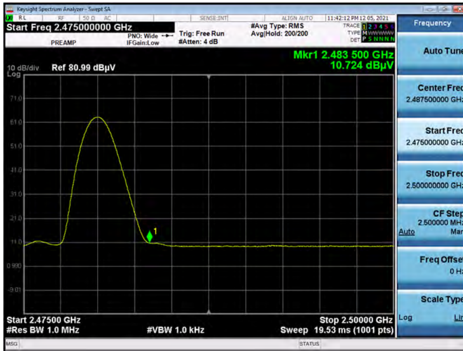
Radiated Restricted Band Edges plot –Peak Result (GFSK, Ch.78, Y-V)
