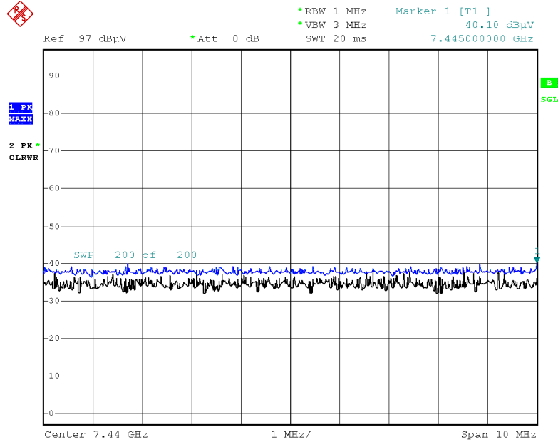
Radiated Spurious Emissions plot – Peak Result (8DPSK, Ch.78 3rd Harmonic, H)
