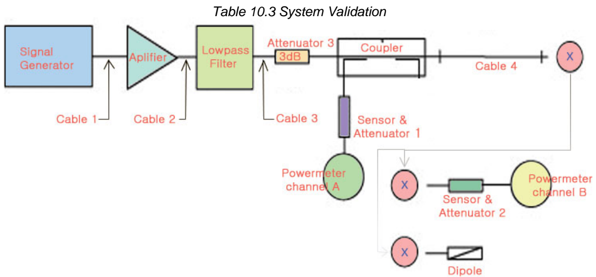
Figure 10.1 Dipole Validation Test Setup
