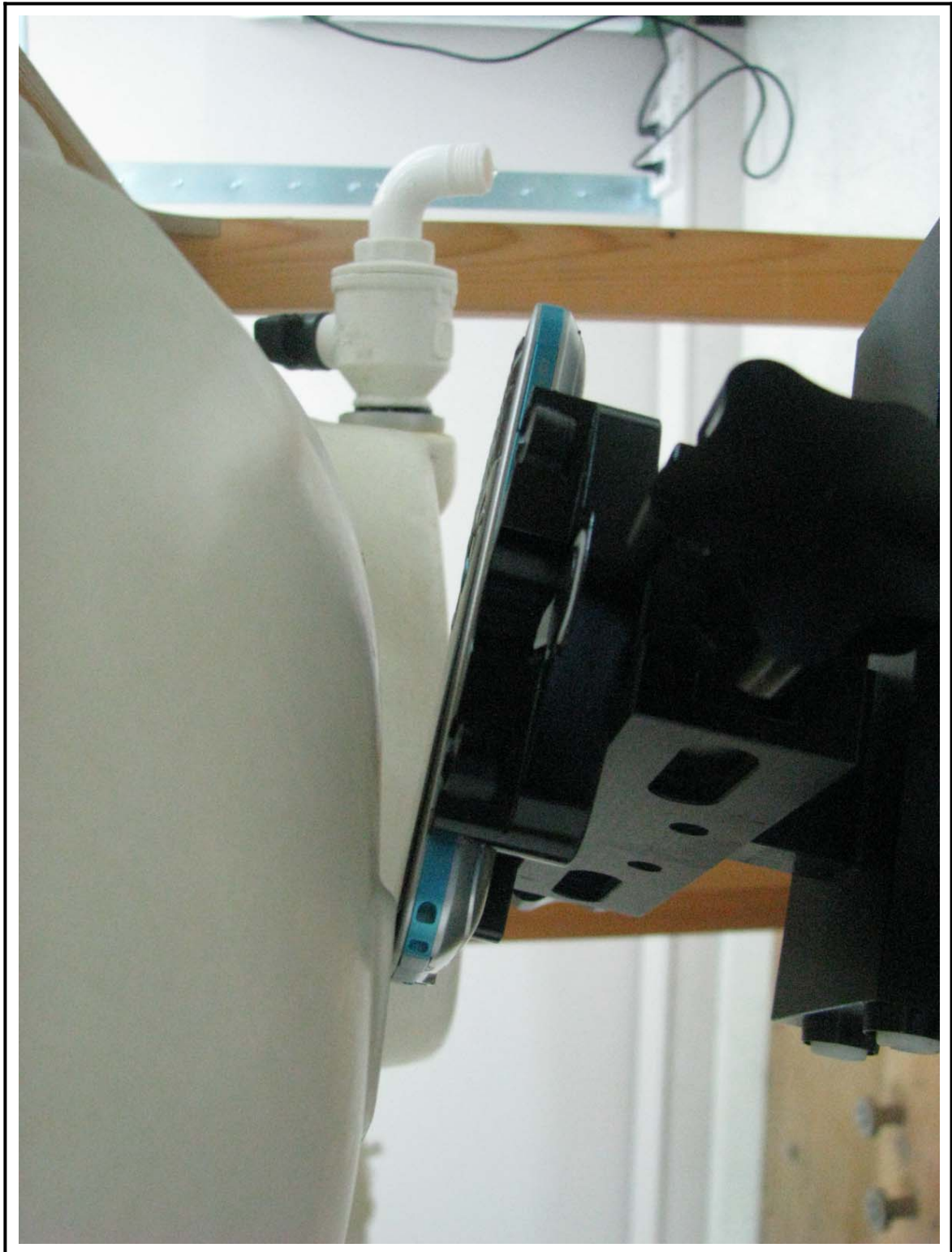
Figure 2 Right Head SAR Test Setup - Ear Tilt Position
