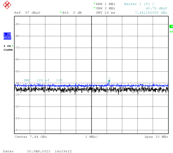
Radiated Spurious Emissions plot – Peak & Average Result (GFSK, Ch.78 3rd Harmonic, H)
