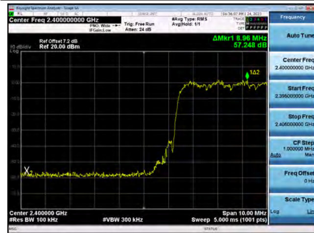
\pi/4 DQPSK(with hopping) Band Edge(CH.0)
