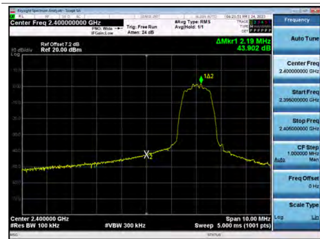
\pi/4 DQPSK(without hopping) Band Edge(CH.0)
