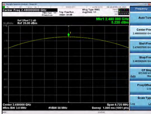
Ant. 2 8DPSK : Peak Power (CH.78)
