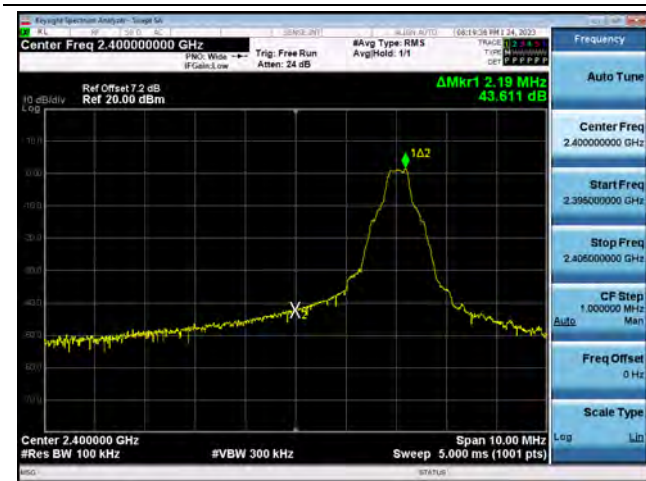
8DPSK(without hopping) Band Edge(CH.0)
