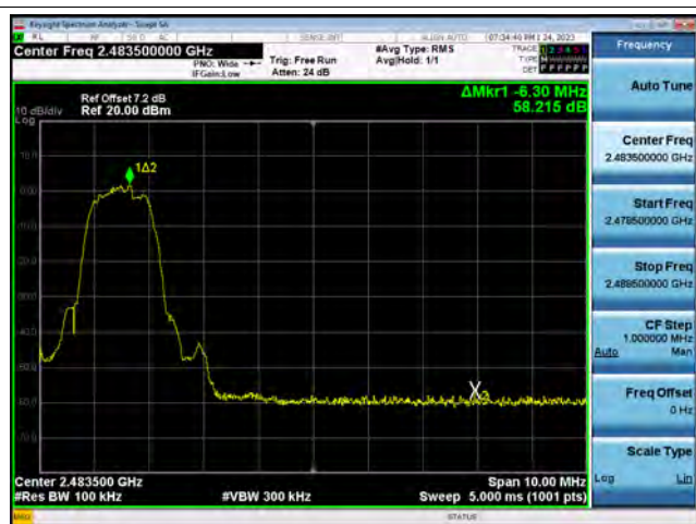
\pi/4 DQPSK (without hopping) Band Edge(CH.78)
