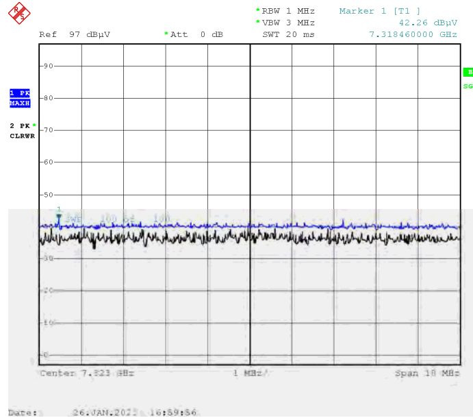
Radiated Spurious Emissions plot – Peak & Average Result ( \pi/4 DQPSK, Ch.39 3rd Harmonic, H)
