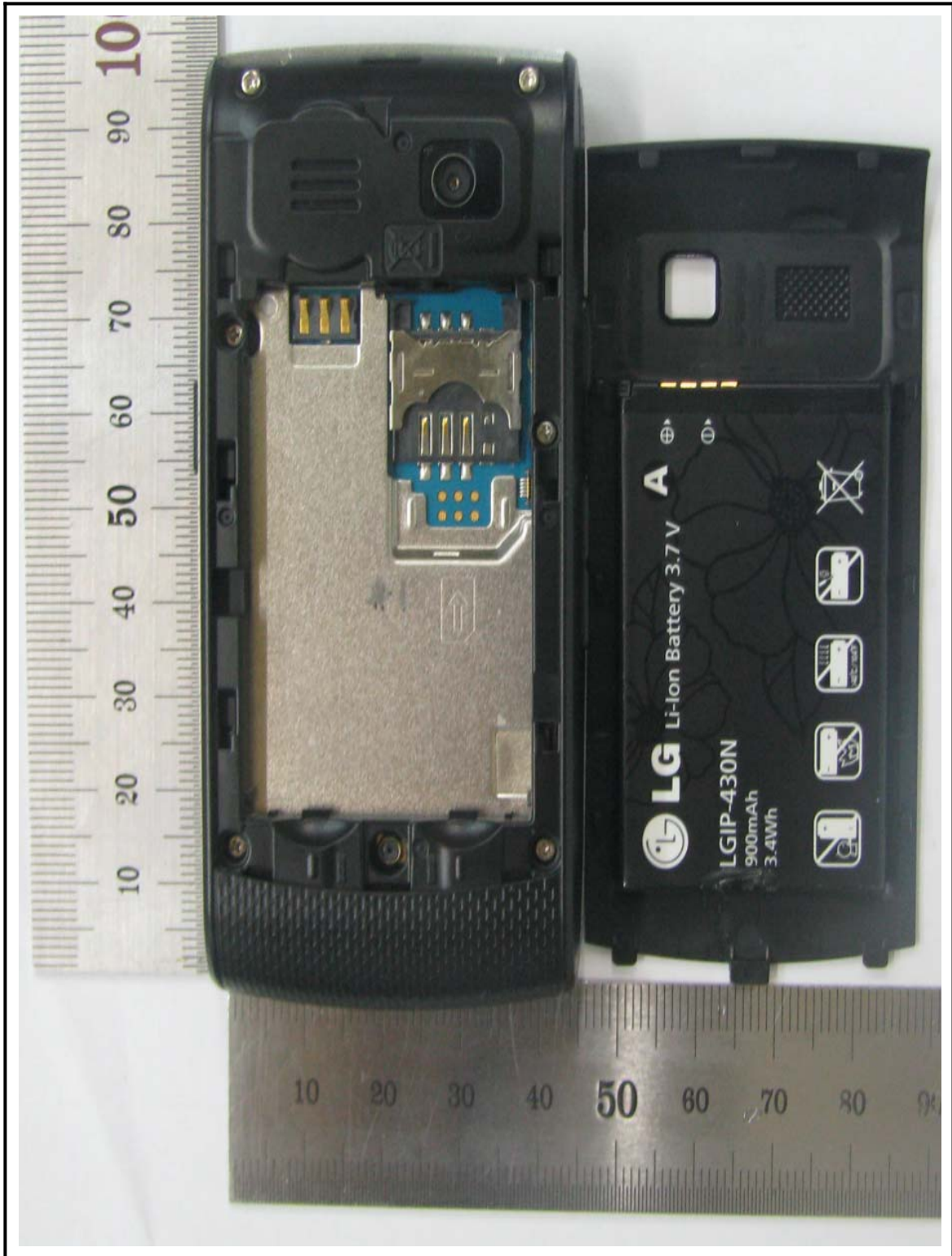
Figure 15 DUT Photo
