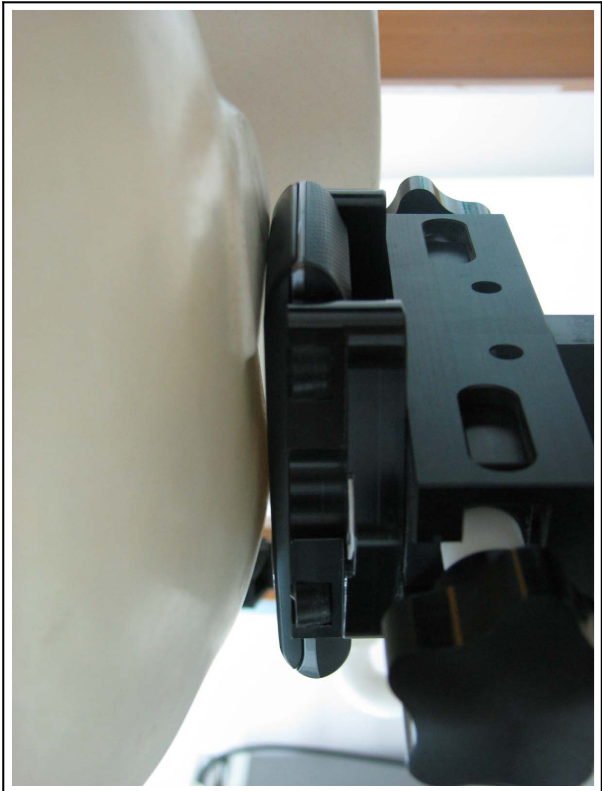
Figure 5 Left Head SAR Test Setup – Cheek Touch Position
