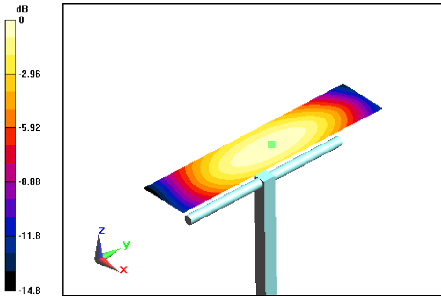
0 dB = 0.481A/m
