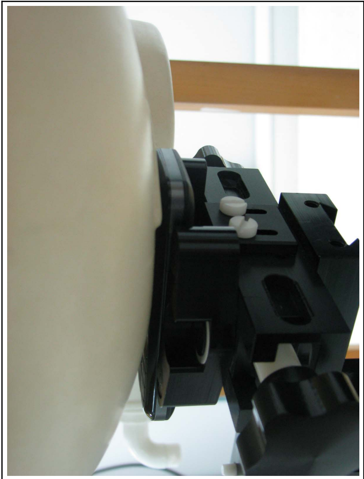
Figure 3 Left Head SAR Test Setup – Cheek Touch Position
