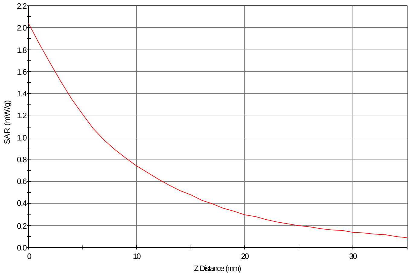
SAR - Z Axis at Hotspot x:67.0 y:6.0
