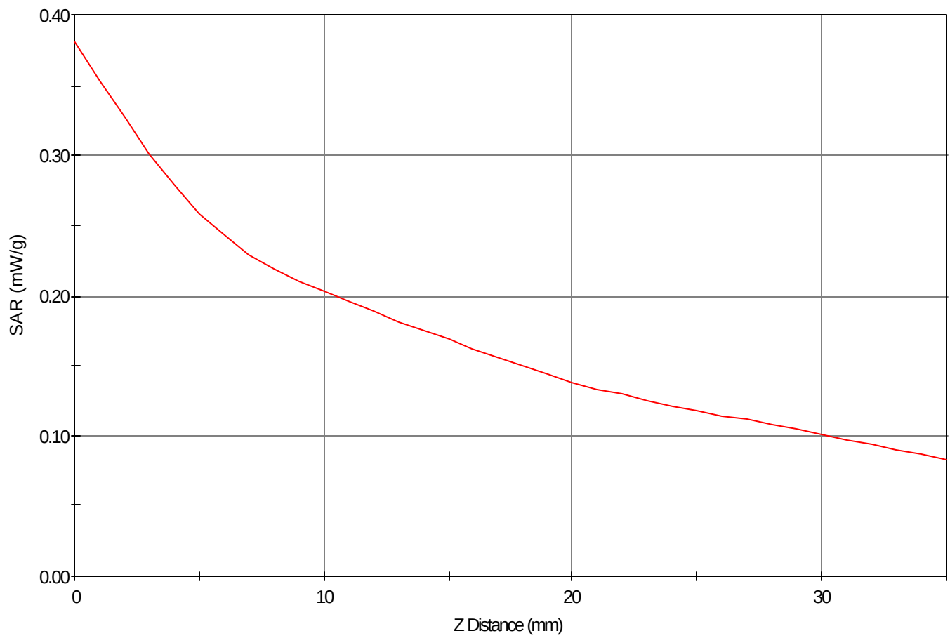
SAR - Z Axis at Hotspot x:55.0 y:17.0
