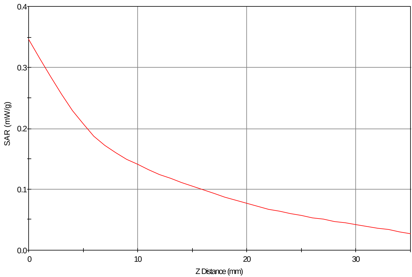
SAR - Z Axis at Hotspot x:-6.0 y:-13.0
