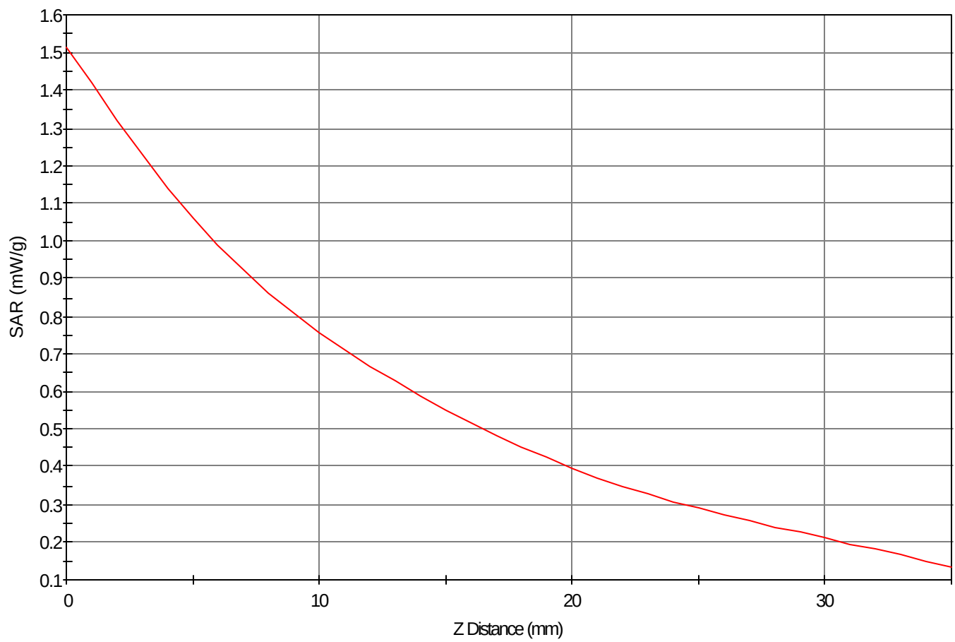
SAR - Z Axis at Hotspot x:70.0 y:15.0
