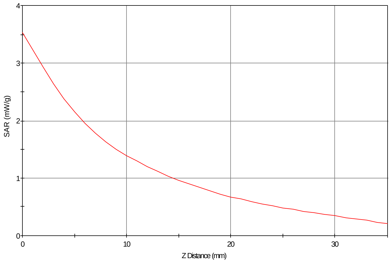
SAR - Z Axis at Hotspot x:11.0 y:-1.0
