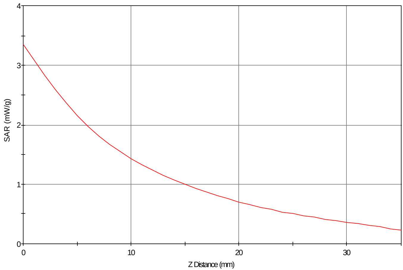
SAR - Z Axis at Hotspot x:12.0 y:0.0
