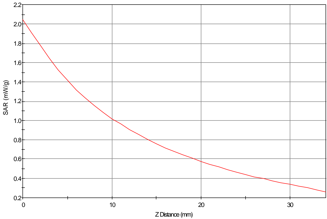
SAR - Z Axis at Hotspot x:87.0 y:19.0
