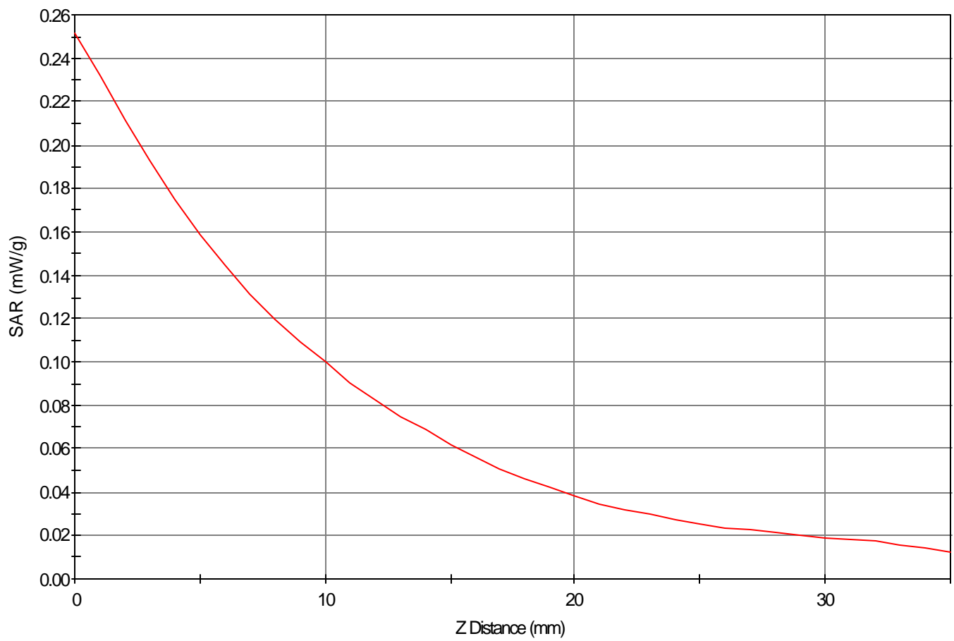
SAR - Z Axis at Hotspot x:103.0 y:-3.0
