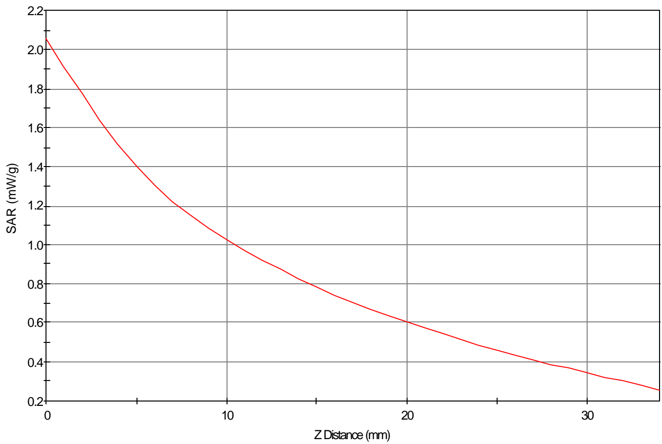
SAR - Z Axis at Hotspot x:83.0 y:7.0
