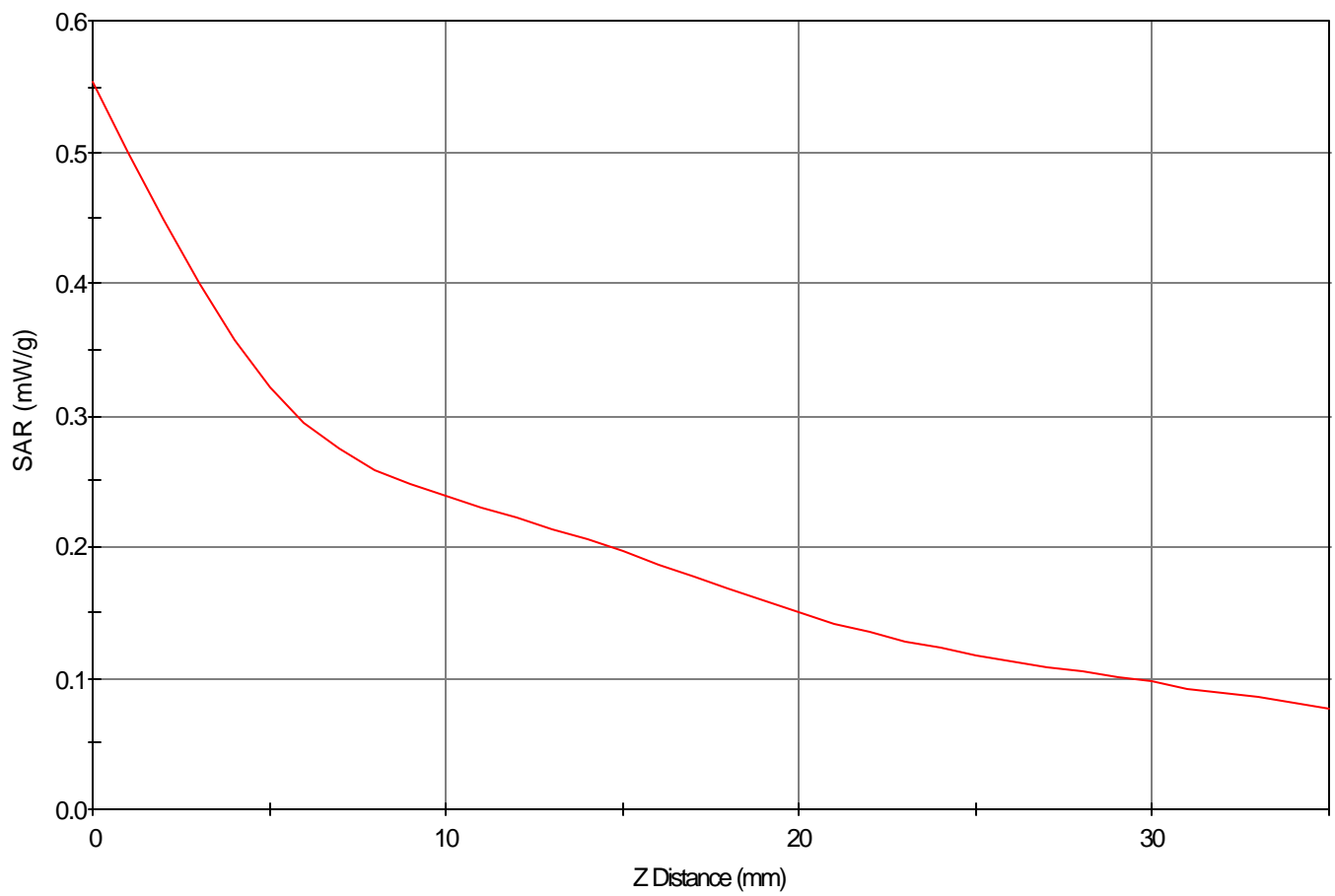
SAR - Z Axis at Hotspot x:69.0 y:8.0
