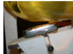
Figure A.12 Left Head SAR Test Setup -- Ear / 15° Tilt Position/ Slide In --
