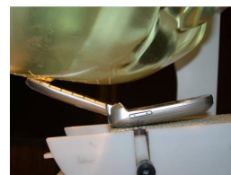
Figure A.2 Right Head SAR Test Setup -- Ear / 15° Tilt Position --
