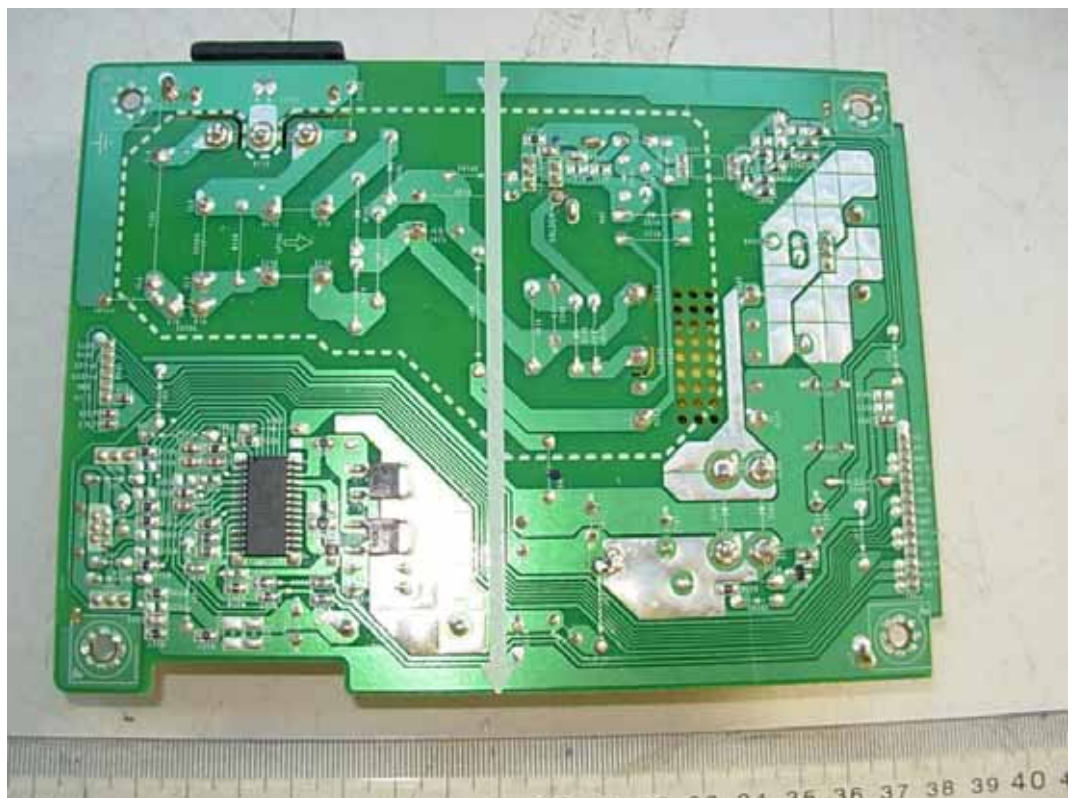
FIGURE 7 LCD MONITOR (M/N: E2711TX) POWER BOARD (SOLDERED SIDE)
