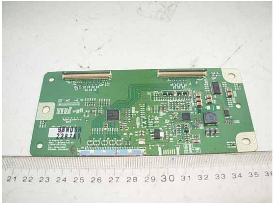
FIGURE 8 LCD MONITOR (M/N: E2711TX) LCD PANEL BOARD #1 (COMPONENT SIDE)
