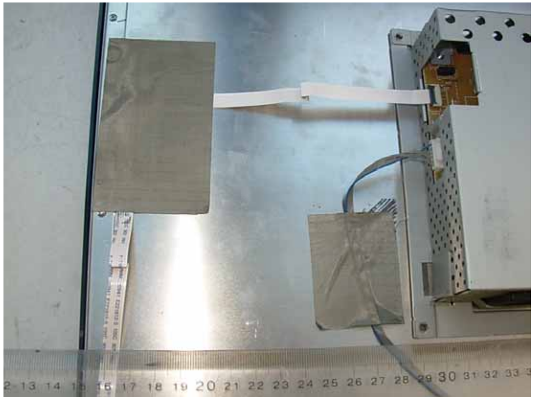
FIGURE 14 LCD MONITOR (M/N: E2711TX) DEBUG #1
