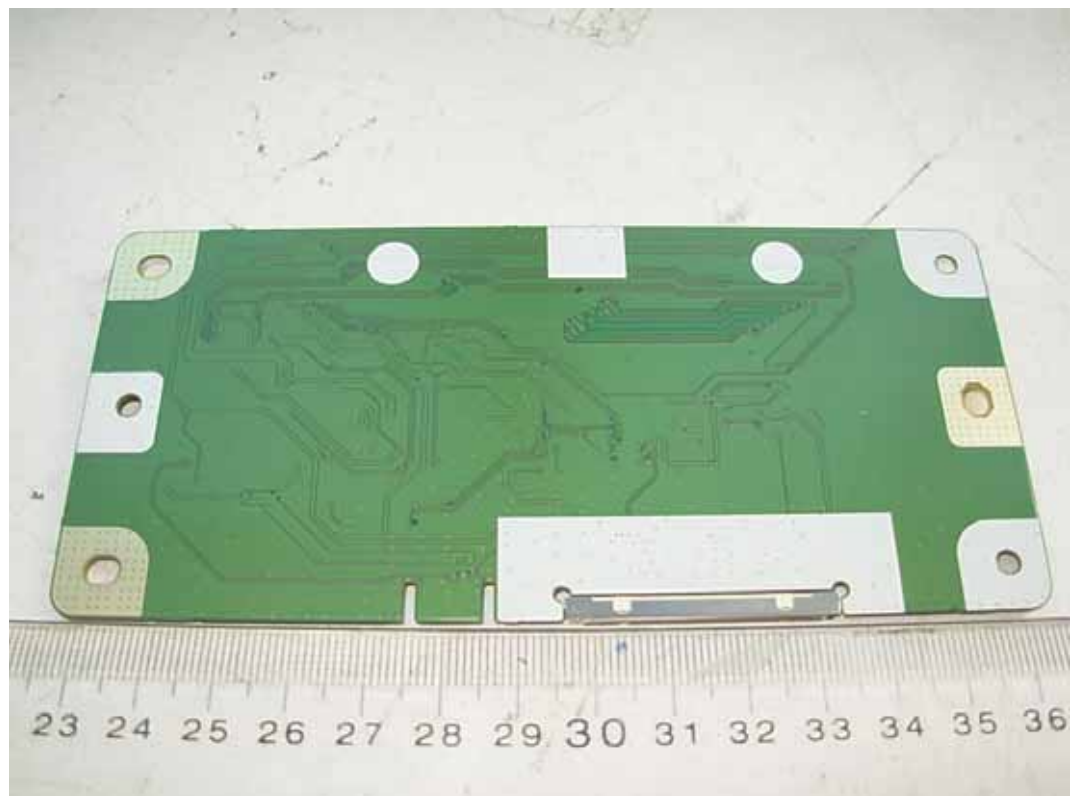
FIGURE 9 LCD MONITOR (M/N: E2711TX) LCD PANEL BOARD #1 BOARD (SOLDERED SIDE)
