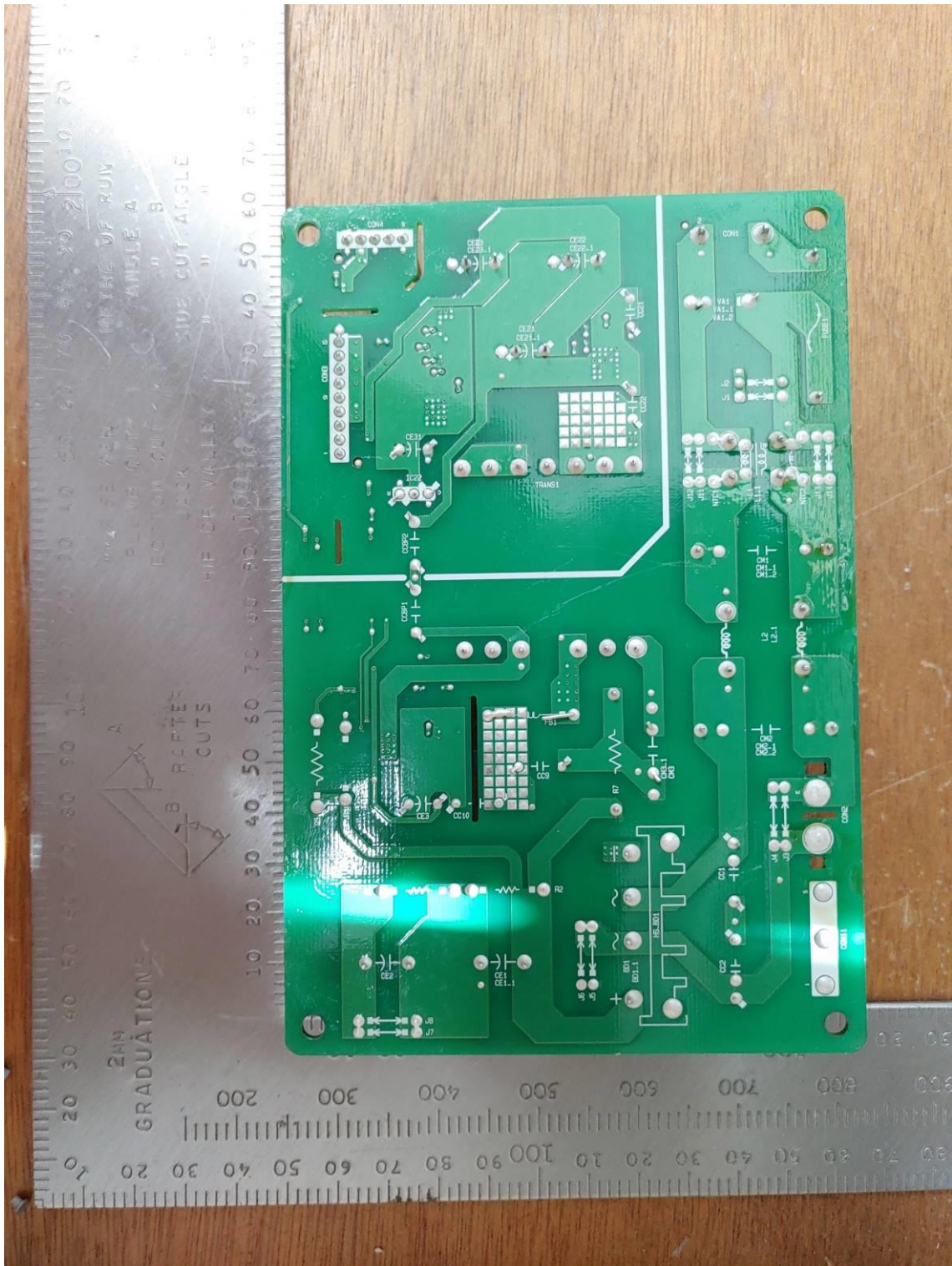
< Power PCB Rear >
