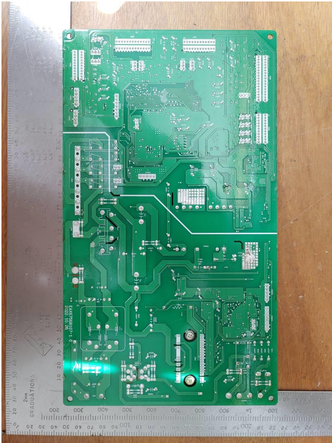
< Main PCB Rear >
