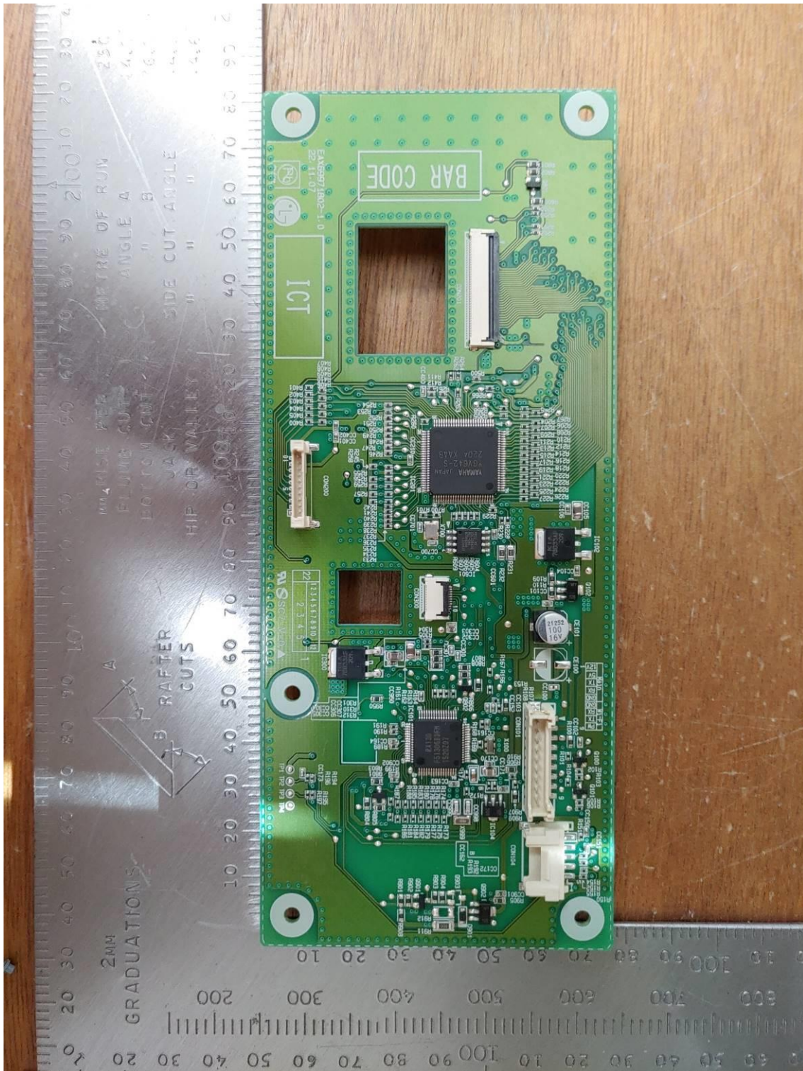
< Display PCB Front
