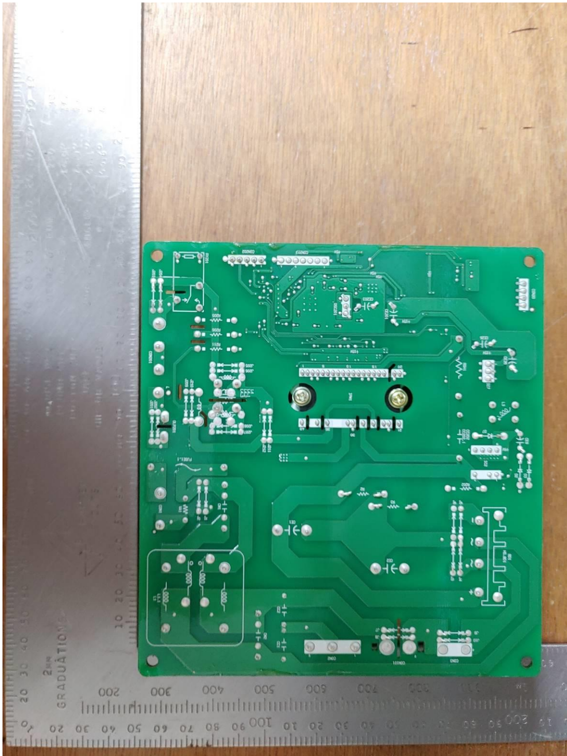
< Comp PCB Rear >
