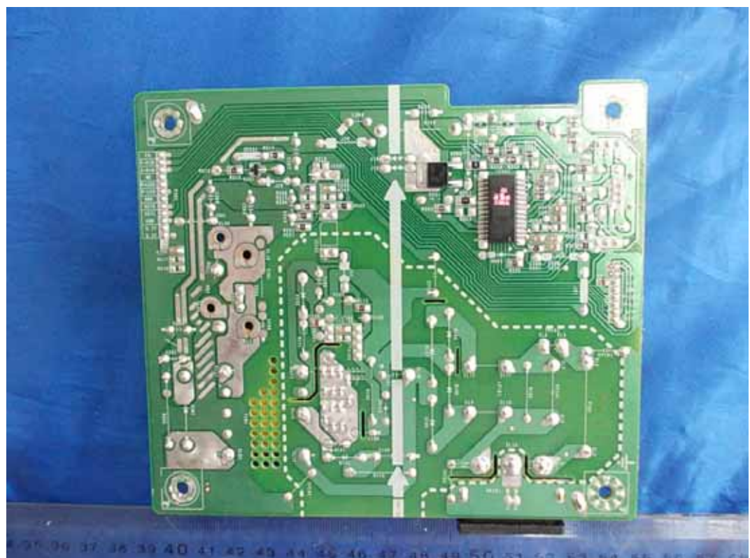
FIGURE 4 LCD MONITOR (M/N: E2411PX) POWER BOARD (SOLDERED SIDE)
