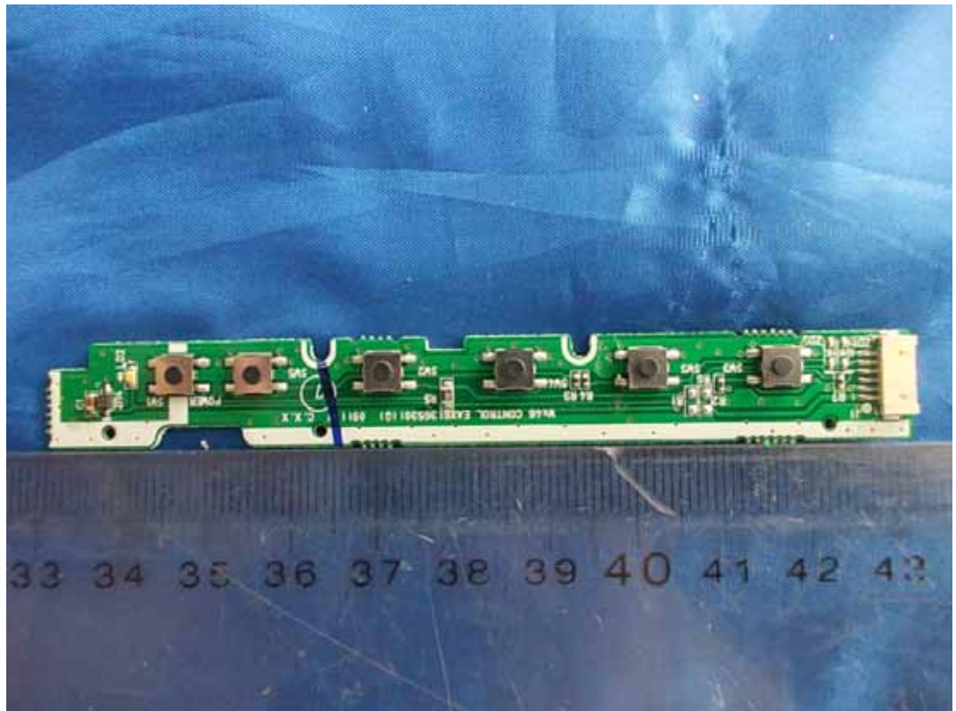
FIGURE 8 LCD MONITOR (M/N: E2411PX) KEY BOARD (COMPONENT SIDE)
