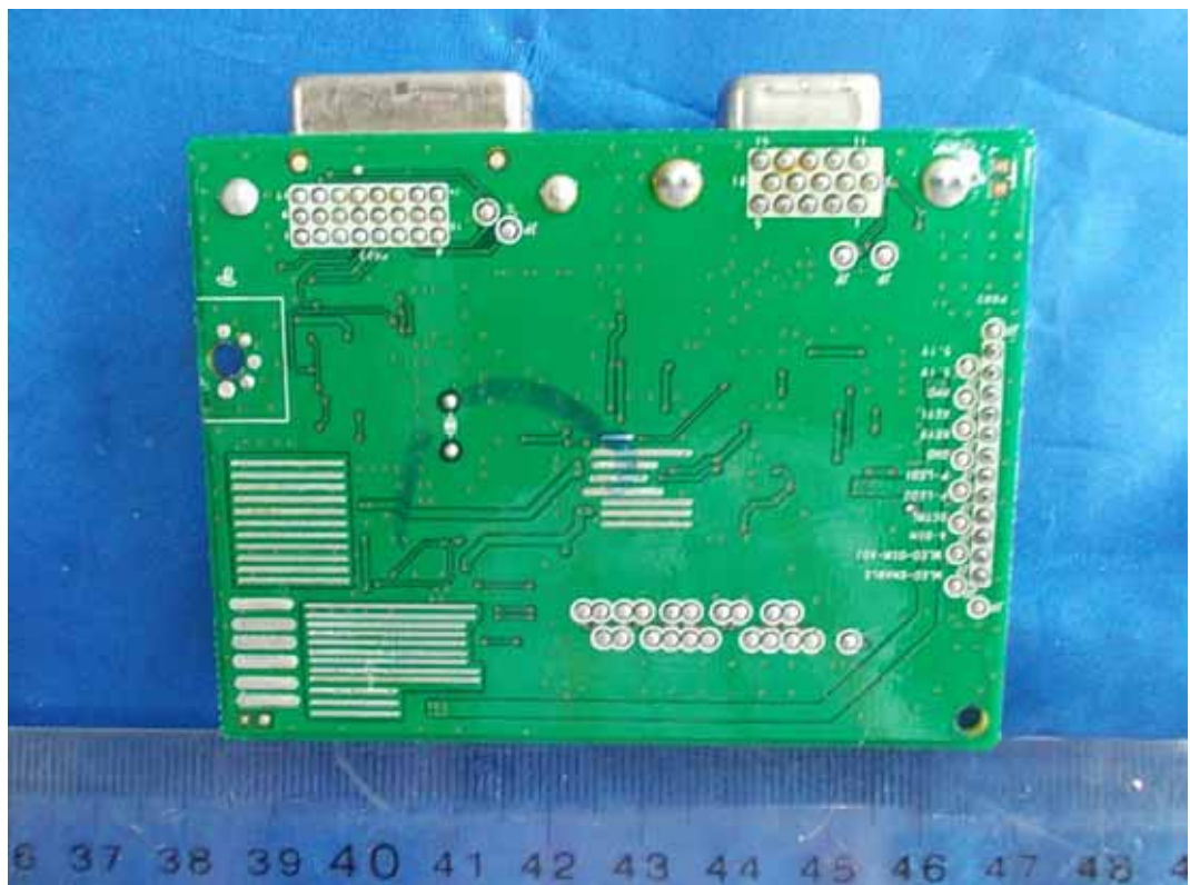
FIGURE 6 LCD MONITOR (M/N: E2411PX) MAIN BOARD (SOLDERED SIDE)
