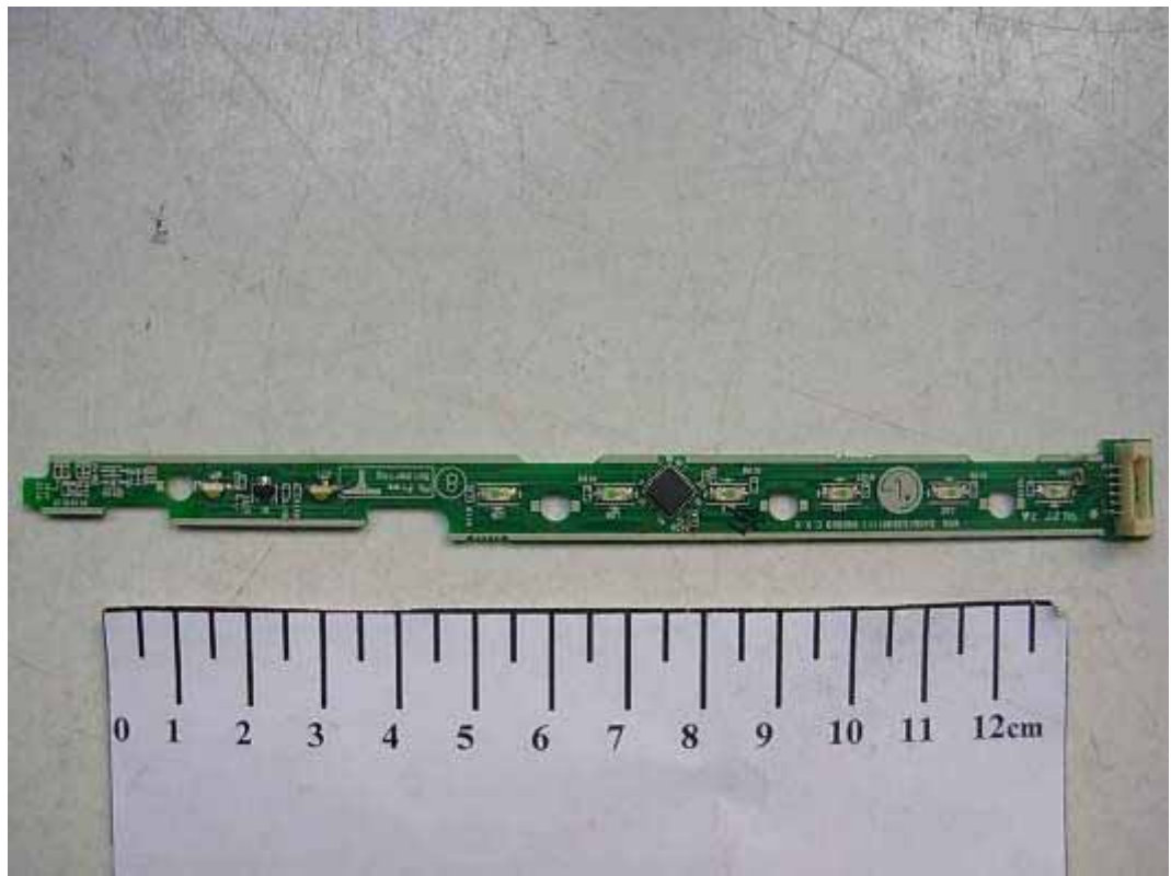
FIGURE 7 LCD MONITOR (M/N: E2350TV) KEY BOARD (COMPONENT SIDE)
