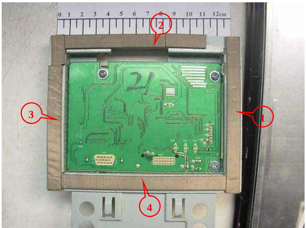
FIGURE 13 LCD MONITOR (M/N: E2350TV) DEBUG #2
