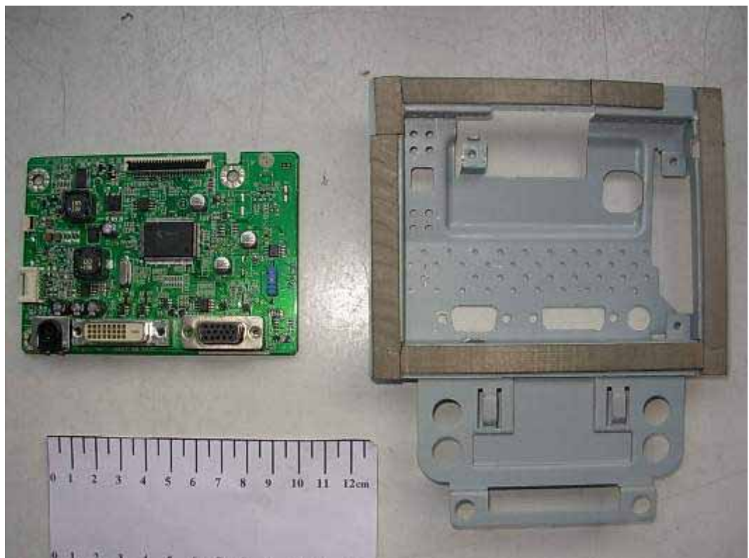
FIGURE 2 LCD MONITOR (M/N: E2350TV) MAIN BOARD COVER REMOVED
