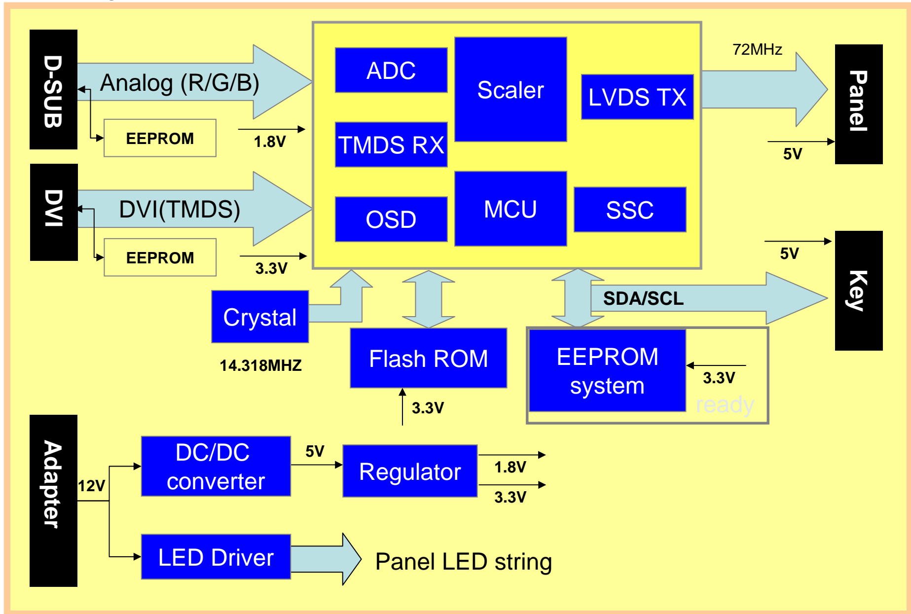
Block diagram for E2340 (NVT)
