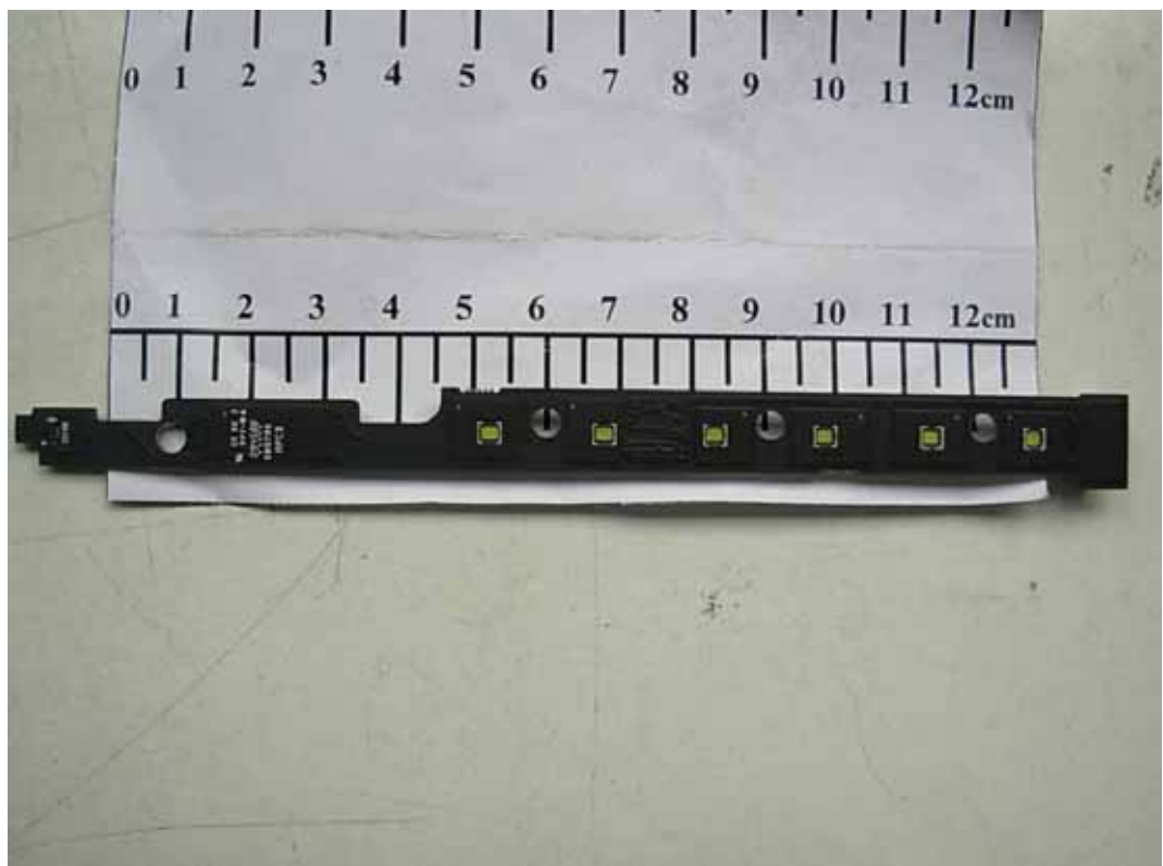
FIGURE 6 LCD MONITOR (M/N: E2250TV) KEY BOARD (SOLDERED SIDE)
