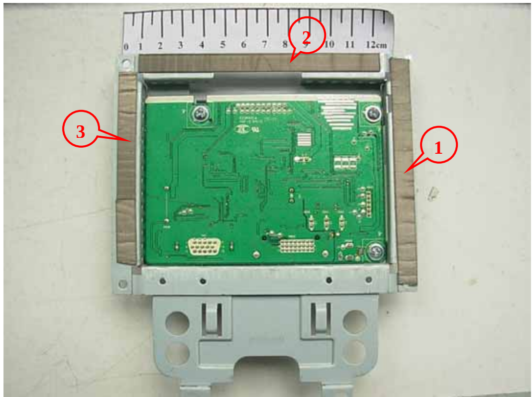
FIGURE 12 LCD MONITOR (M/N: E2250TV) DEBUG #3
