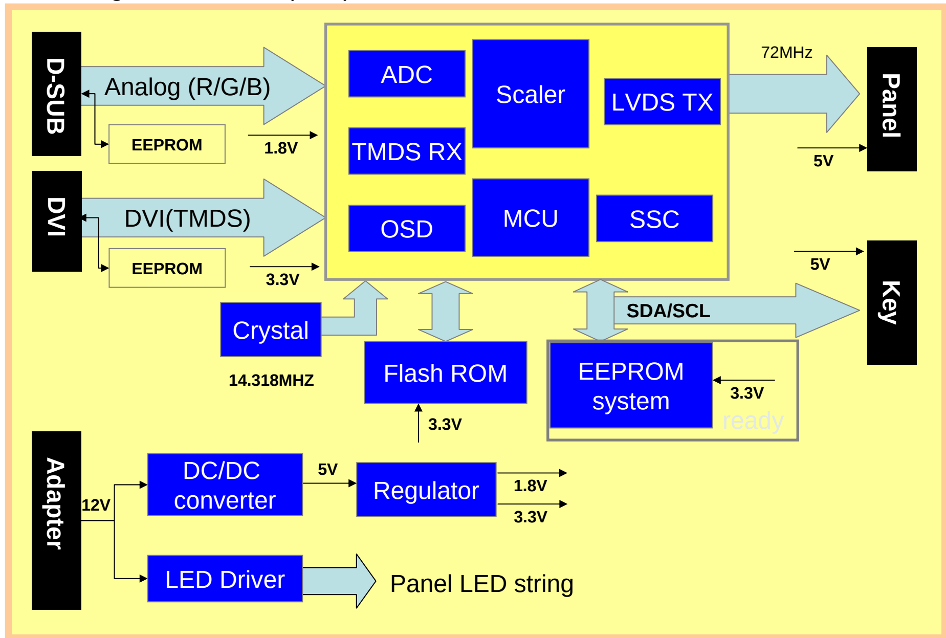
Block diagram for E2240 (NVT)
