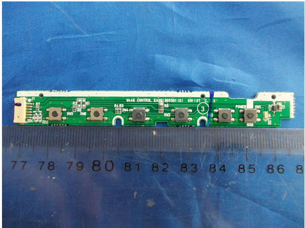
FIGURE 8 LCD MONITOR (M/N: E2211PX) KEY BOARD (COMPONENT SIDE)
