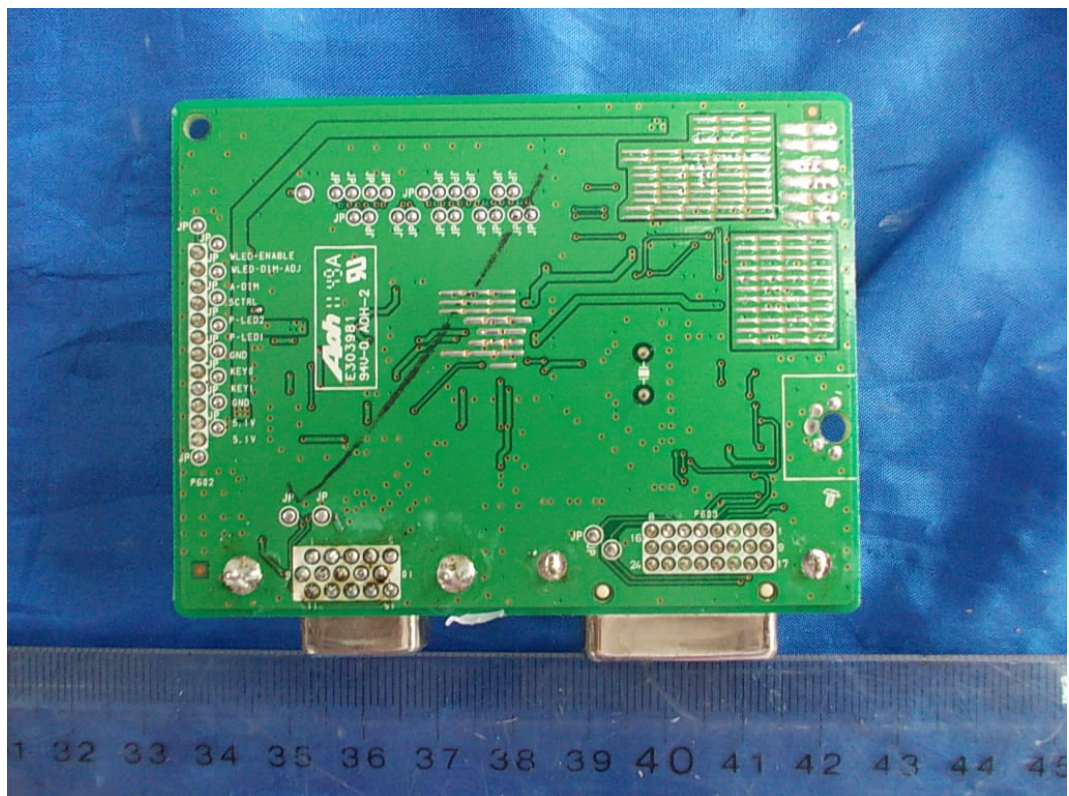
FIGURE 6 LCD MONITOR (M/N: E2211PX) MAIN BOARD (SOLDERED SIDE)
