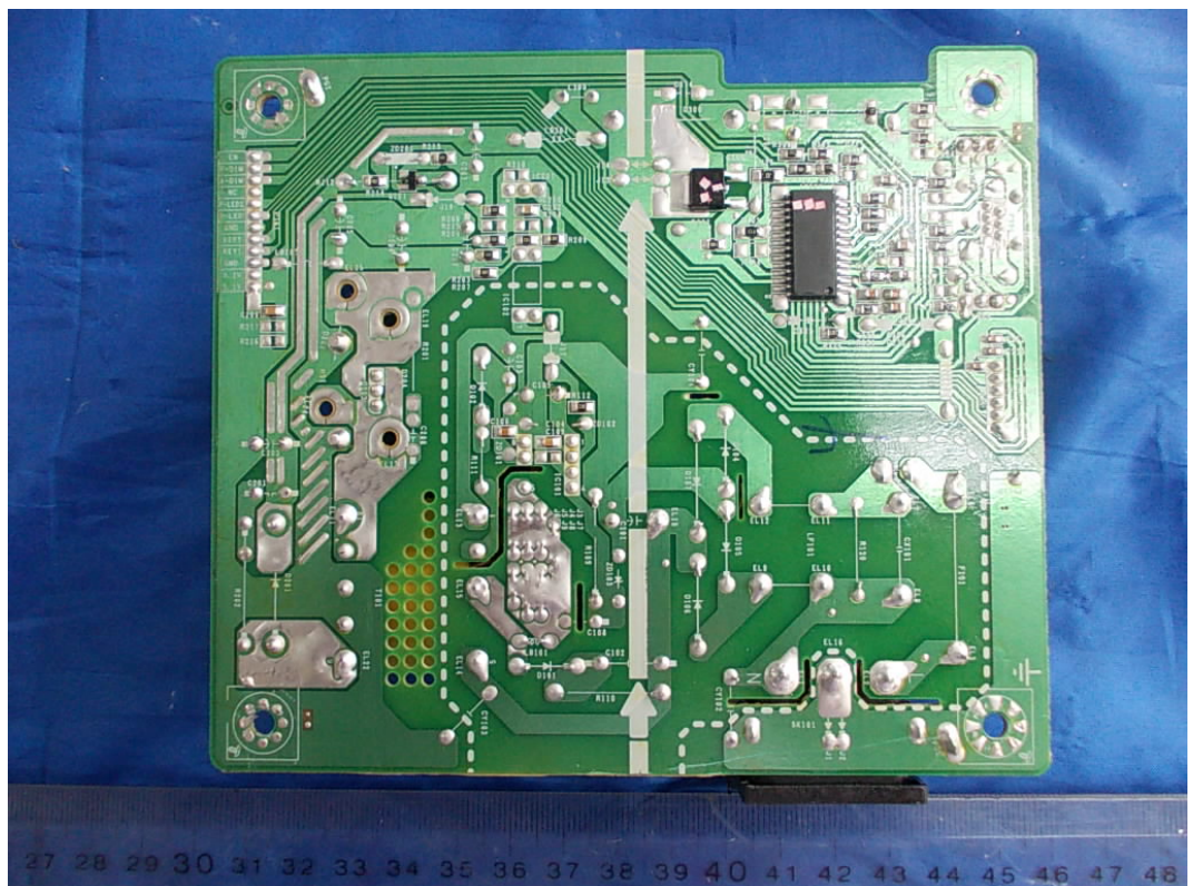
FIGURE 4 LCD MONITOR (M/N: E2211PX) POWER BOARD (SOLDERED SIDE)
