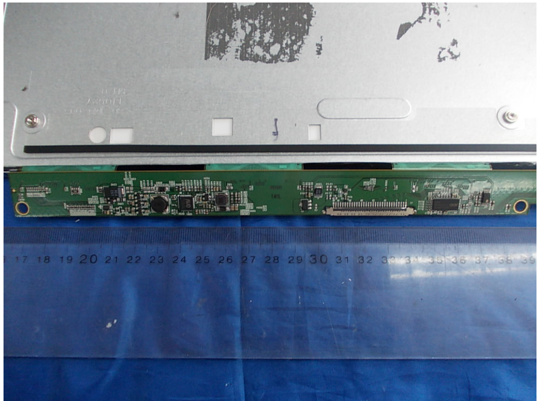
FIGURE 10 LCD MONITOR (M/N: E2211PX) LCD PANEL BOARD (COMPONENT SIDE-1)
