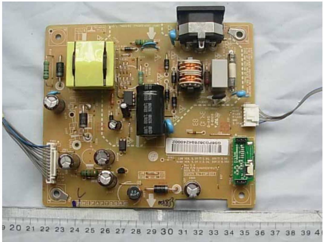
FIGURE 10 LCD MONITOR (M/N: E2210PW) POWER BOARD (COMPONENT SIDE)
