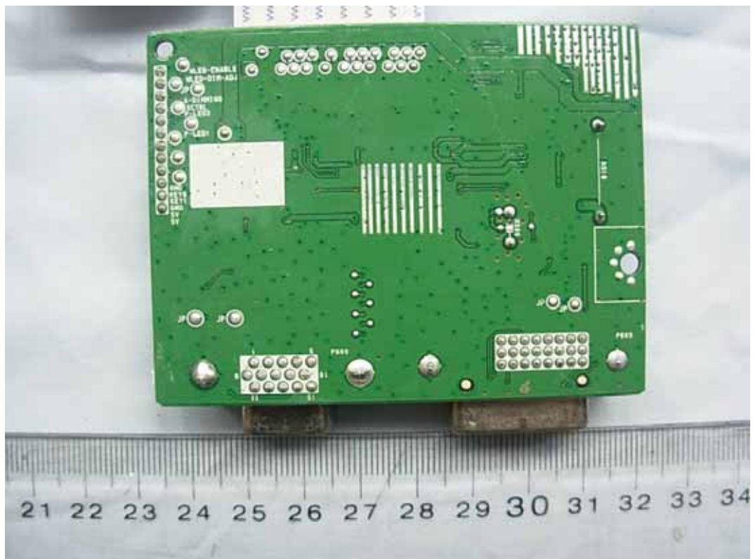
FIGURE 8 LCD MONITOR (M/N: E2210PW) MAIN BOARD (SOLDERED SIDE)
