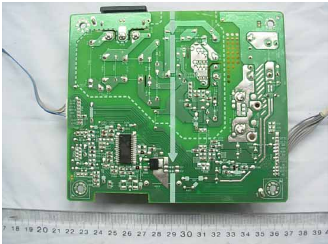
FIGURE 11 LCD MONITOR (M/N: E2210PW) POWER BOARD (SOLDERED SIDE)
