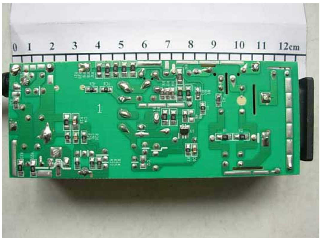
FIGURE 20 LCD MONITOR (M/N: E2050TV) ADAPTER #2 (MAIN BOARD – SOLDERED SIDE)
