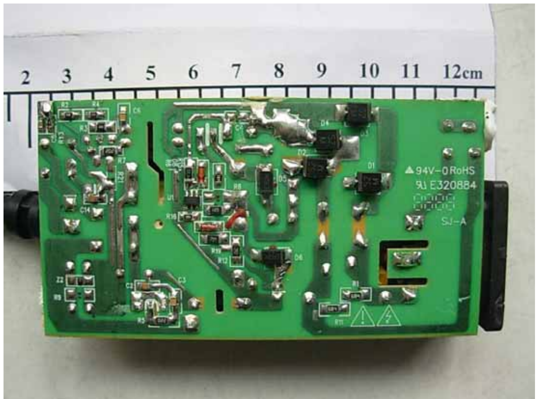
FIGURE 14 LCD MONITOR (M/N: E2050TV) ADAPTER #1 (MAIN BOARD – SOLDERED SIDE)
