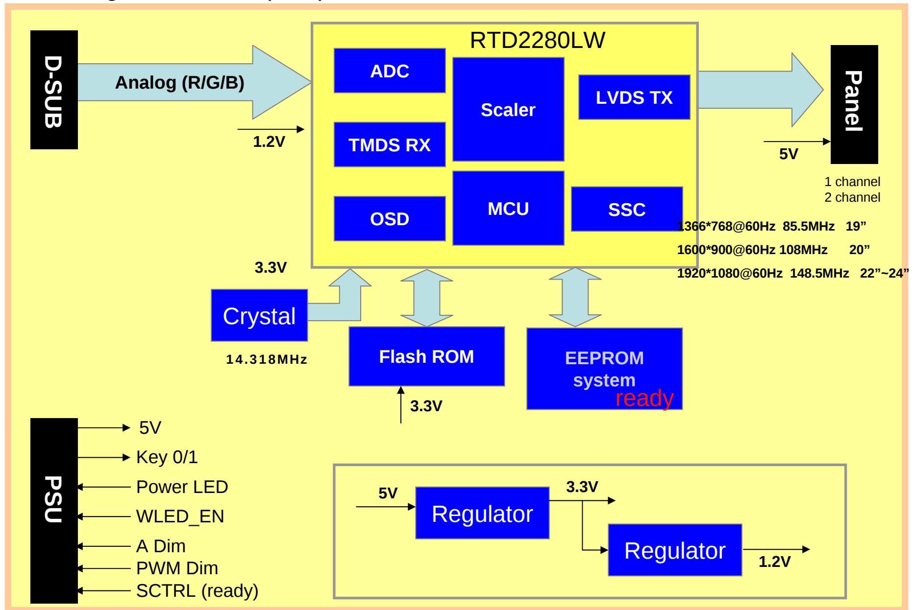
Block diagram for E41S (RTK)
