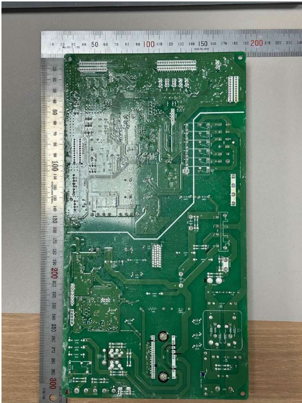
Alternated New Item_<Main PCB Section-2>
