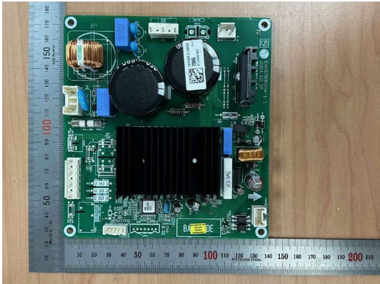
Alternated New Item_<Sub PCB Section-1>
