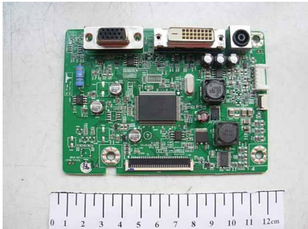
FIGURE 3 LCD MONITOR (M/N: E1950TV) MAIN BOARD (COMPONENT SIDE)
