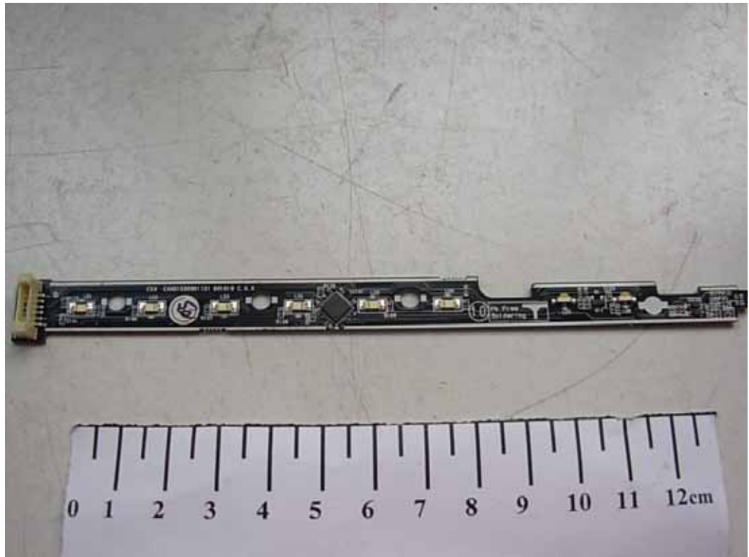
FIGURE 6 LCD MONITOR (M/N: E1950TV) KEY BOARD (COMPONENT SIDE)
