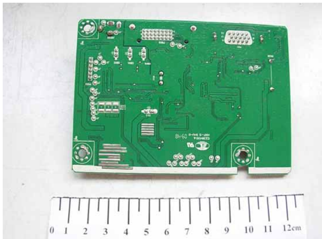
FIGURE 4 LCD MONITOR (M/N: E1950TV) MAIN BOARD (SOLDERED SIDE)
