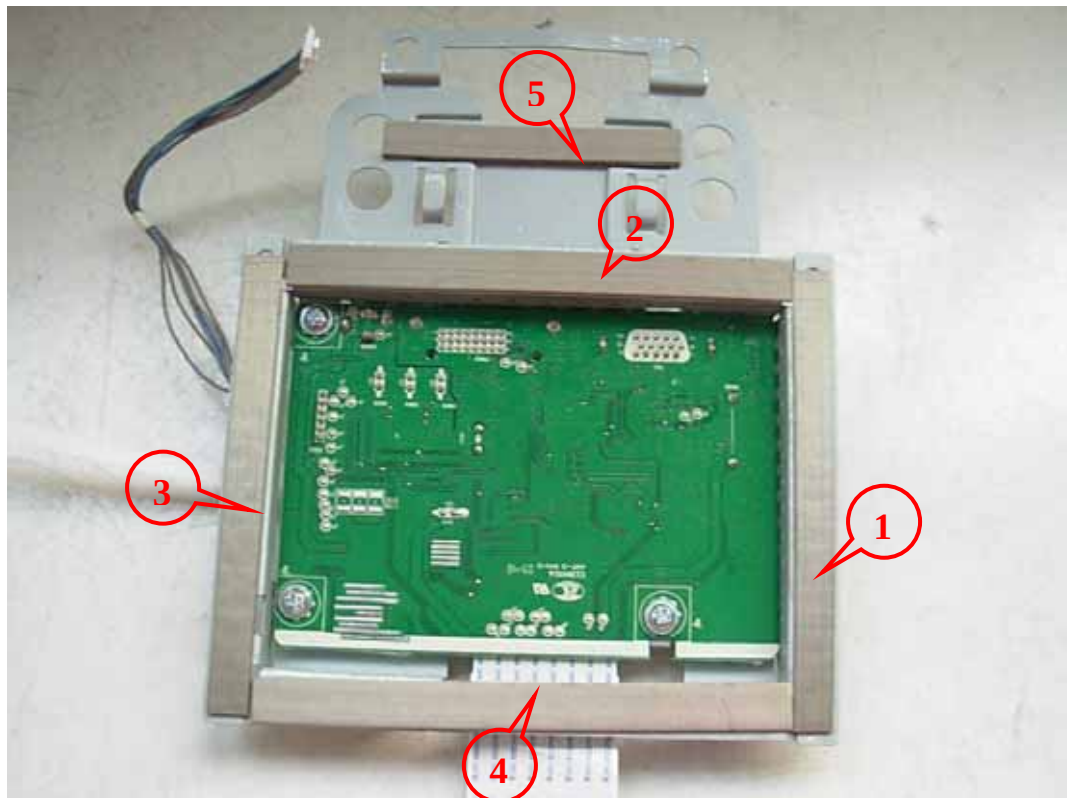
FIGURE 11 LCD MONITOR (M/N: E1950TV) DEBUG
