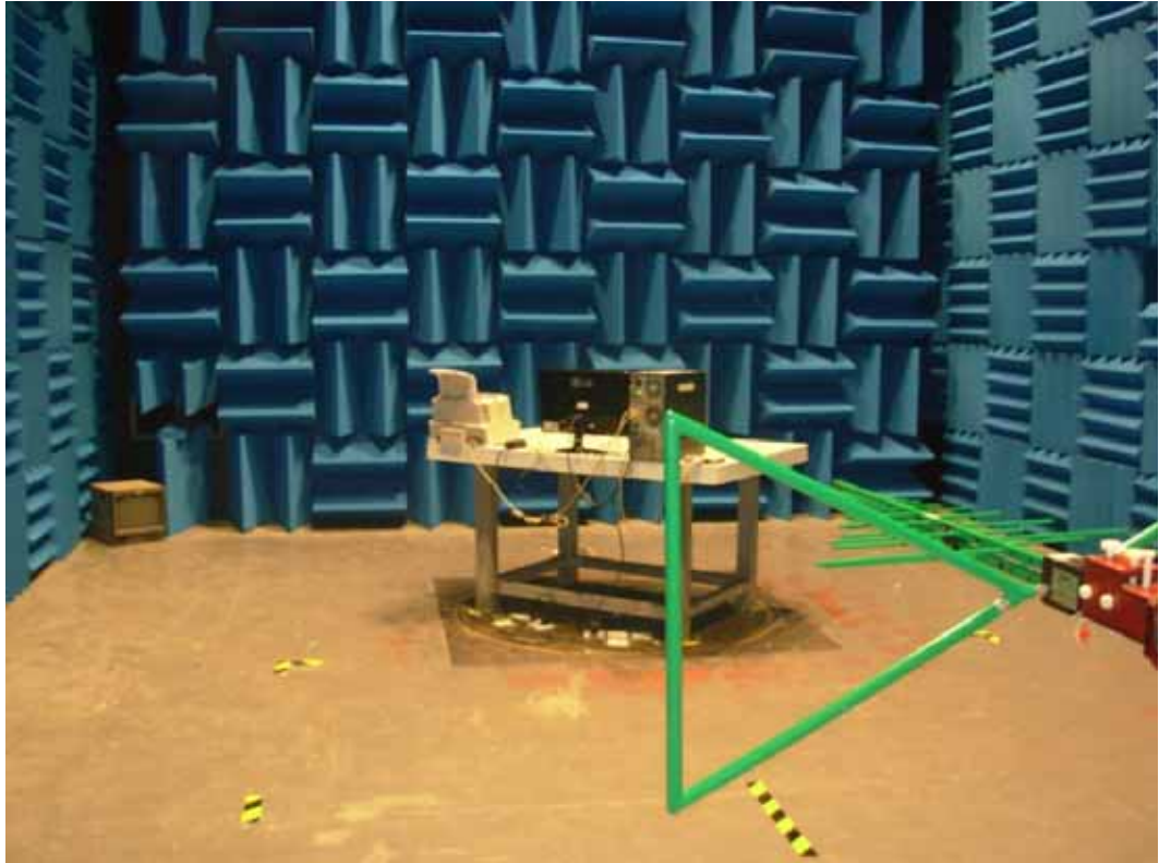
SETUP WITH MAXIMUM DETECTED EMISSION AT HORIZONTAL POLARIZATION (TEST MODE: D-SUB 640*480@60Hz) (ADAPTER: DSA-36W-12 1 24)
