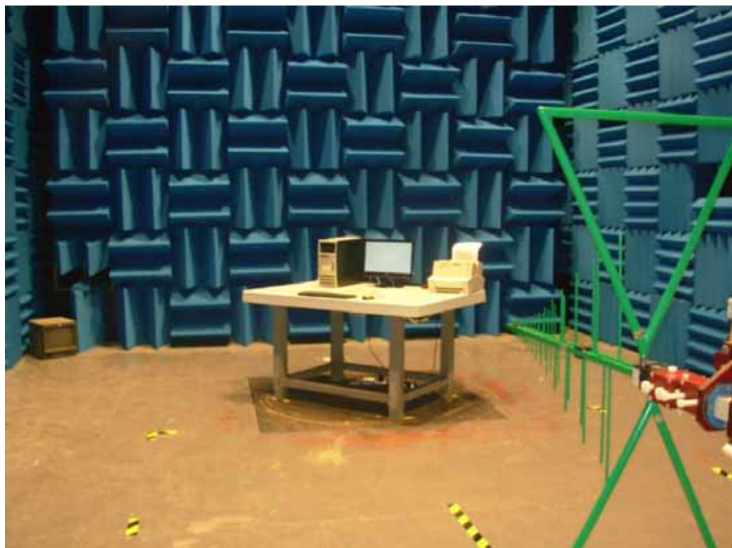
SETUP WITH MAXIMUM DETECTED EMISSION AT VERTICAL POLARIZATION (TEST MODE: D-SUB 640*480@60Hz) (ADAPTER: DSA-36W-12 1 24)
