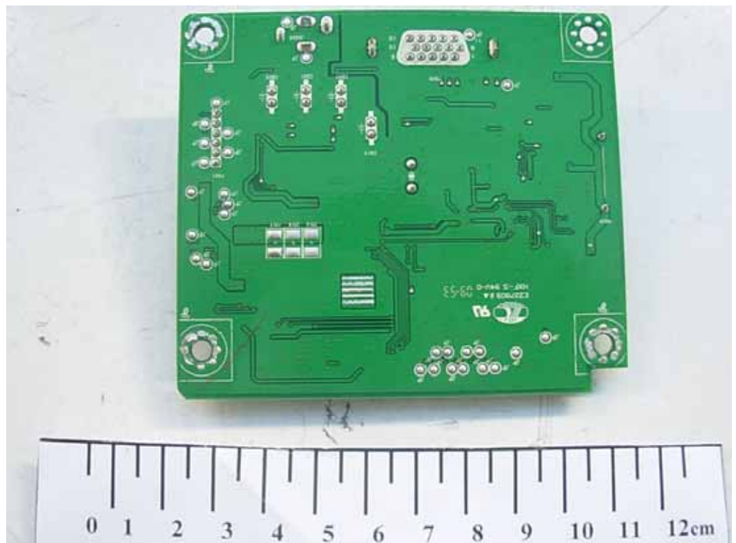
FIGURE 5 LCD MONITOR (M/N: E1950SV) MAIN BOARD (SOLDERED SIDE)
