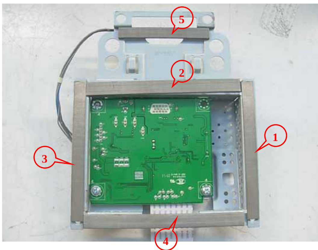
FIGURE 10 LCD MONITOR (M/N: E1950SV) DEBUG
