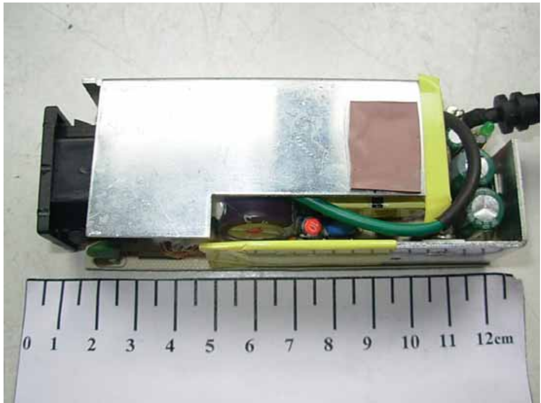
FIGURE 18 LCD MONITOR (M/N: E1950SV) ADAPTER #2 (MAIN BOARD – COMPONENT SIDE)
