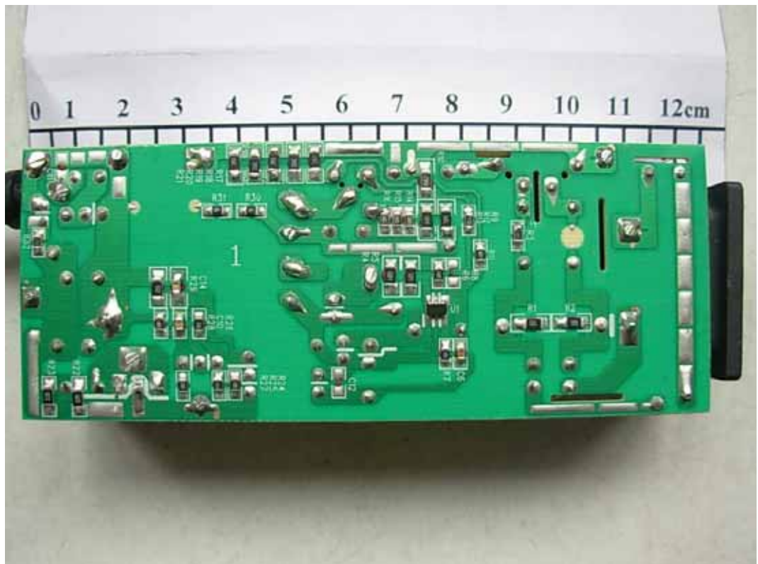
FIGURE 19 LCD MONITOR (M/N: E1950SV) ADAPTER #2 (MAIN BOARD – SOLDERED SIDE)
