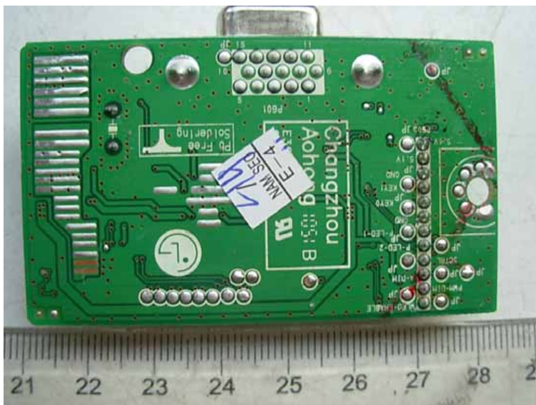
FIGURE 4 LCD MONITOR (M/N: E1641SX) MAIN BOARD (COMPONENT SIDE)
