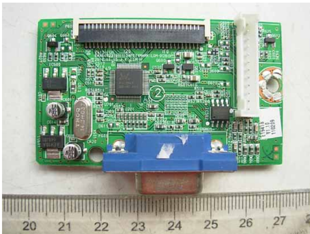
FIGURE 3 LCD MONITOR (M/N: E1641SX) MAIN BOARD (COMPONENT SIDE)
