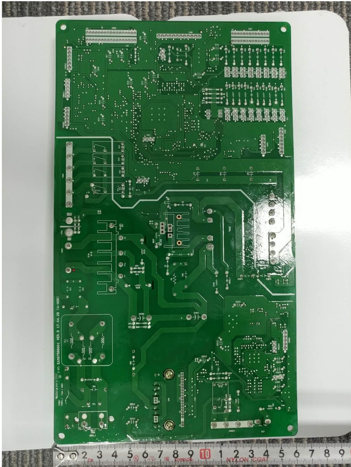
< Main PCB >
