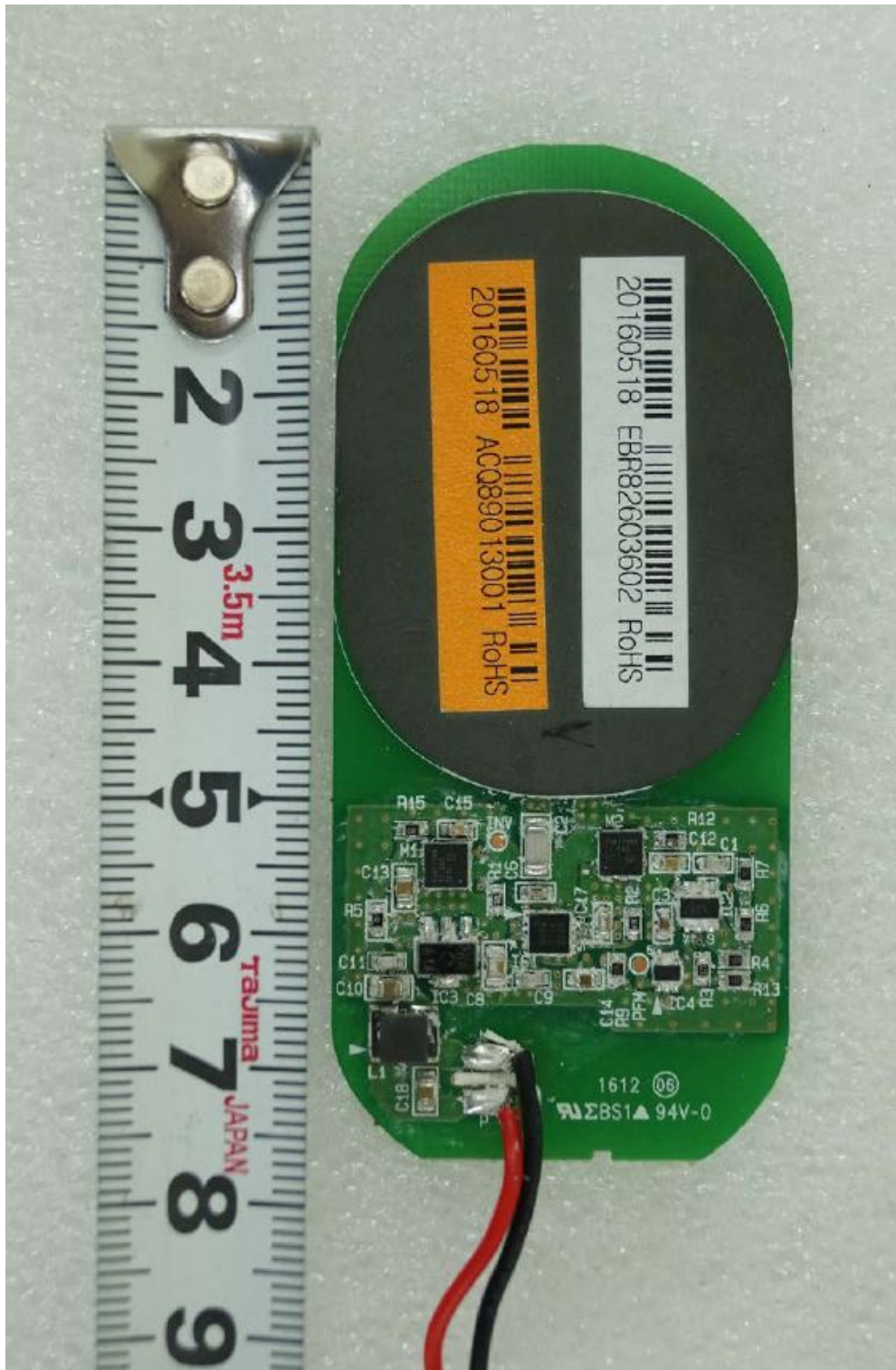
<Wireless shelf module -1>
