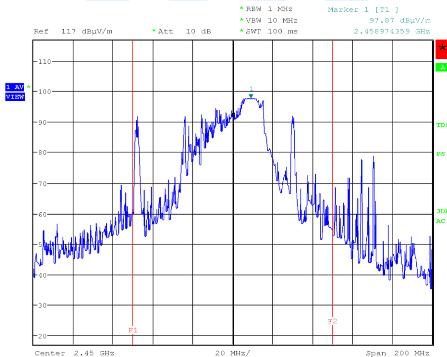
< Fig 10. Frequency Measurements _Load (Minimum Frequency Observed: 2.458 GHz) >
