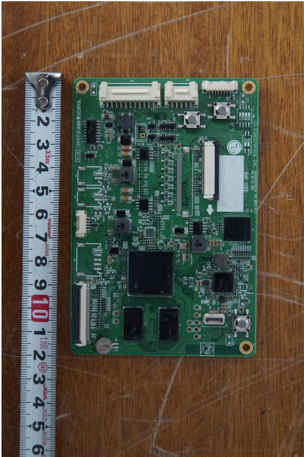
< PCB Section_Alternated New LCD PCB_ P/No. : EBR40225613 >
