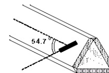
Δ - BEAM Fig 4-3 Triangular Probe Configuration
