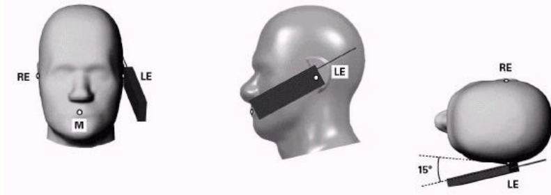
Fig 9-3 Front, Side and Top View of Ear/15° Tilt Position
