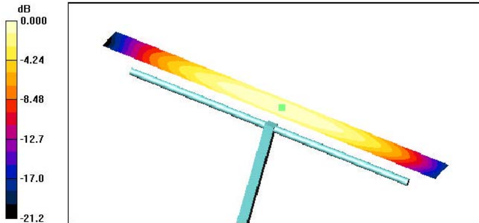
0 dB = 0.441A/m
