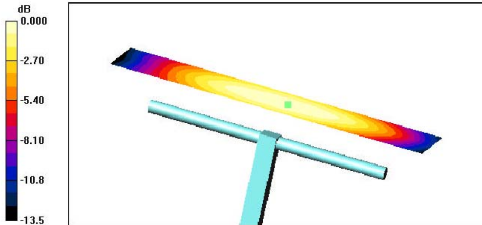
0 dB = 0.412A/m
