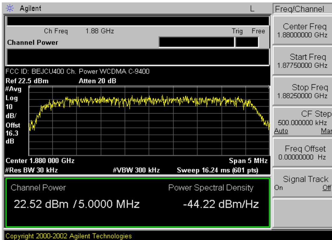
Plot A-20. Channel Power Plot (PCS WCDMA Mode – Ch. 9400)
