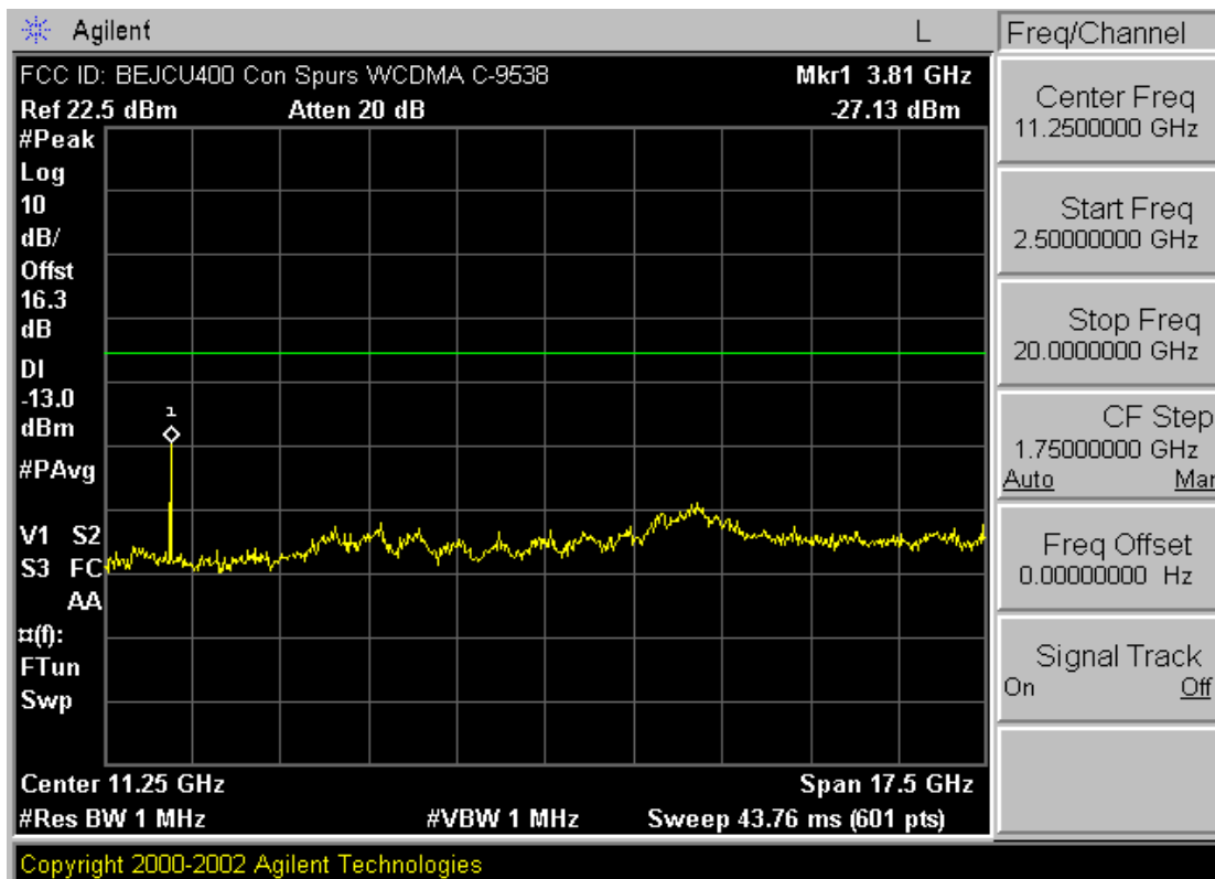
Plot A-22. Conducted Spurious Plot (PCS WCDMA Mode – Ch. 9538)
