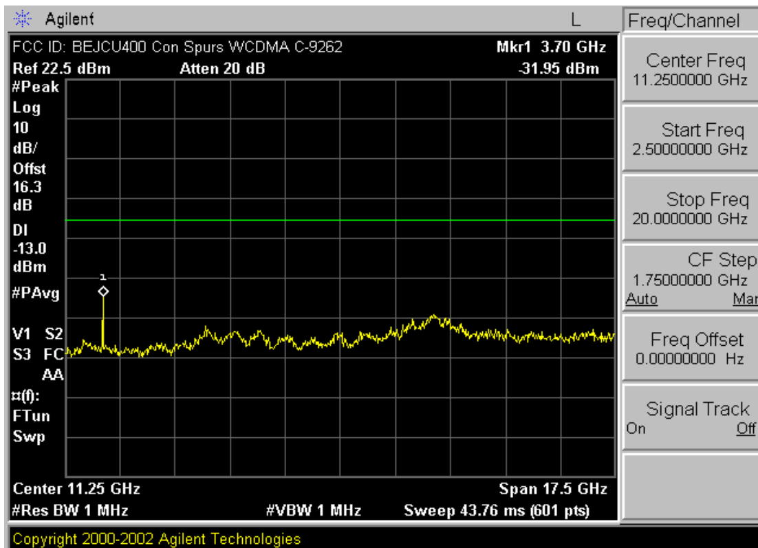
Plot A-14. Conducted Spurious Plot (PCS WCDMA Mode – Ch. 9262)
