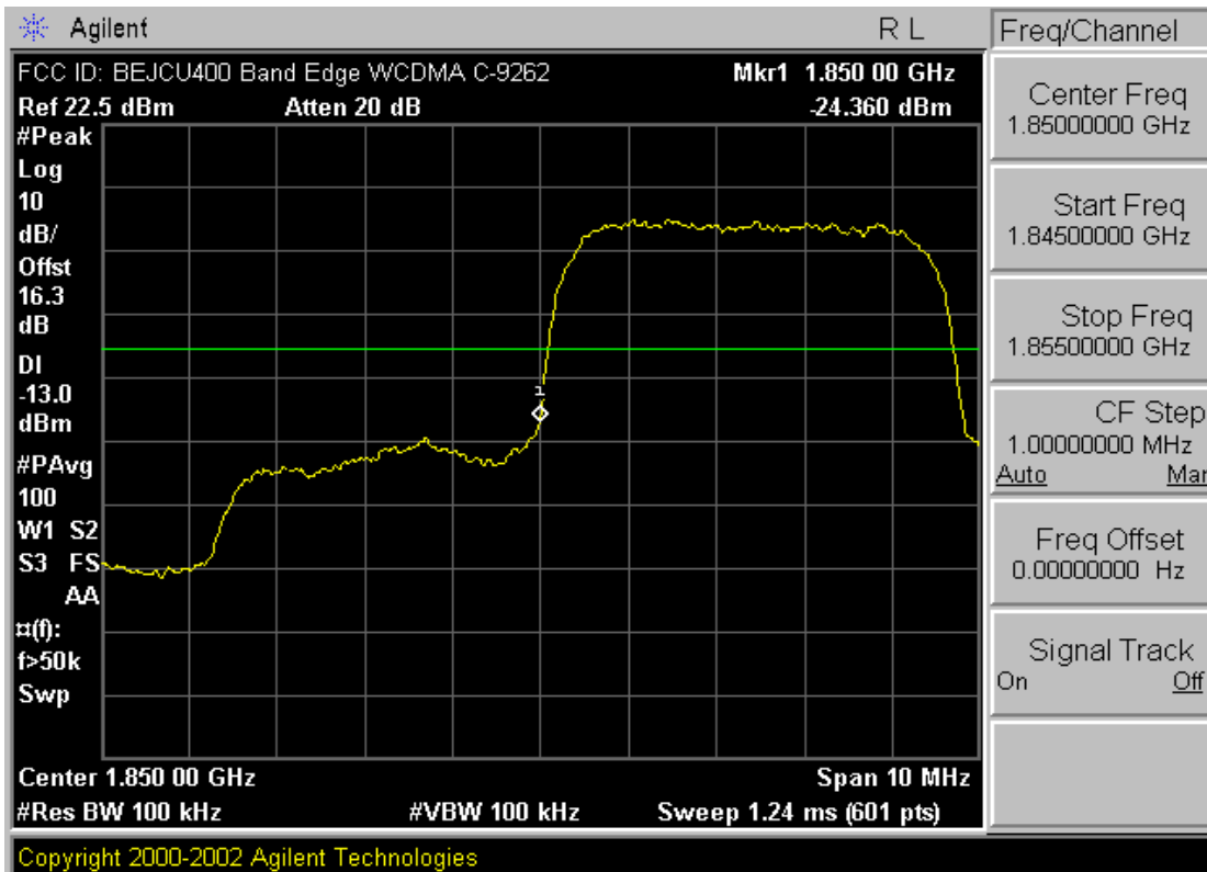
Plot A-15. Band Edge Plot (PCS WCDMA Mode – Ch. 9262)
